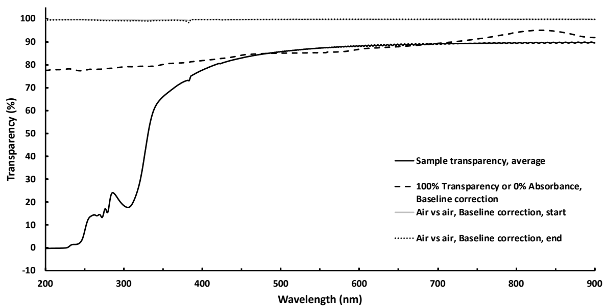
Figure S13. Optical transmission of PC- h measured on a 32 μm thick film.
