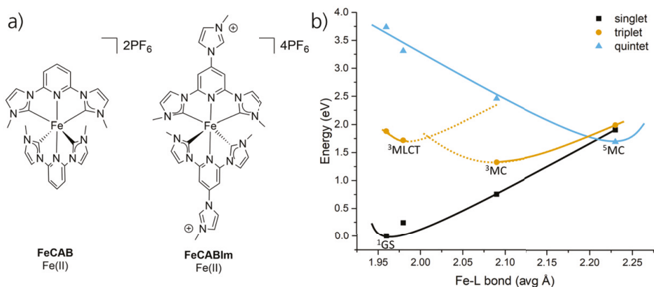
Figure 3.4: a) Molecular structure FeCAB discussed in papers I–IV, together with FeCABIm discussed in paper I. b) Projected potential energy surfaces showing the relevant excited state landscape for FeCABIm. Points are calculated by DFT at the B3LYP* level of theory, lines represent a guide to the interpretation.
