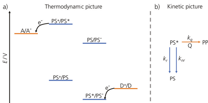
Figure 4.3: Illustration of a) the thermodynamic picture versus b) the kinetic picture of bimolecular charge-transfer. The excited photosensitiser PS^* is quenched by an acceptor A or donor D (collectively called quenchers, Q) to form photoproducts PP. The quenching rate k_Q will compete with the intramolecular deactivation rates k_r (radiative) and k_{nr} (non-radiative).
