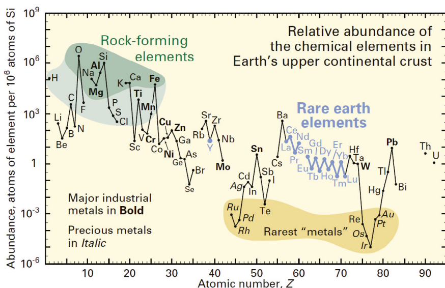
Figure 2.10: An overview of the abundance of all elements present in Earth's crust. On the vertical axis abundance is plotted on a logarithmic scale, normalised to Si. On the horizontal axis the atomic number of the element is plotted. The figure is courtesy of the U.S. Geological Survey.[59]
