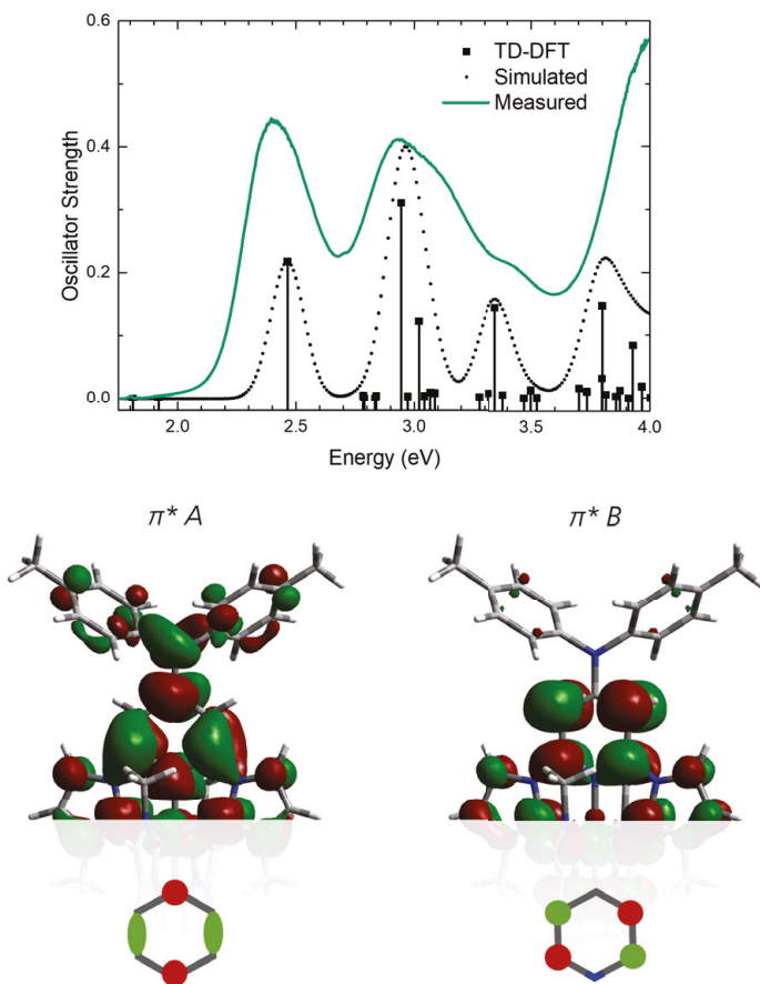
Figure 3.10: Absorption spectrum of FeCABCN1 compared to a simulated absorption spectrum calculated by TD-DFT at the B3LYP* level of theory (corrected by -0.16 eV). Below is a representation of the relevant NTOs of different symmetries, here called \pi^* A and \pi^* B .
