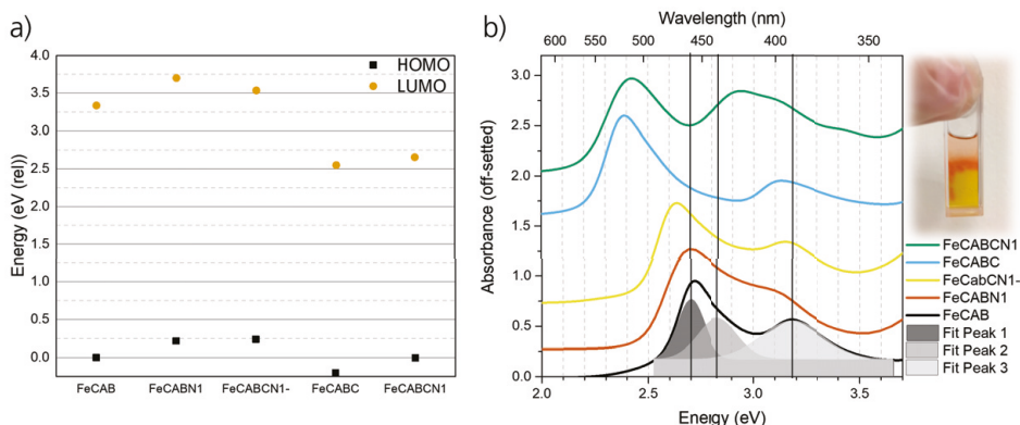
Figure 3.9: a) Relative HOMO and LUMO energies for FeCABCN1 with related complexes. The HOMO energy of FeCAB is used as a reference point to which 0 eV is assigned. Calculated by DFT at the B3LYP* level of theory. b) Compared absorption spectra for the same set of complexes, off-setted and scaled to facilitate qualitative comparison. A Gaussian fit to the absorption spectrum of FeCAB is shown by filled contours. The inset shows the colour change of FeCABCN1 as it changes protonation state.
