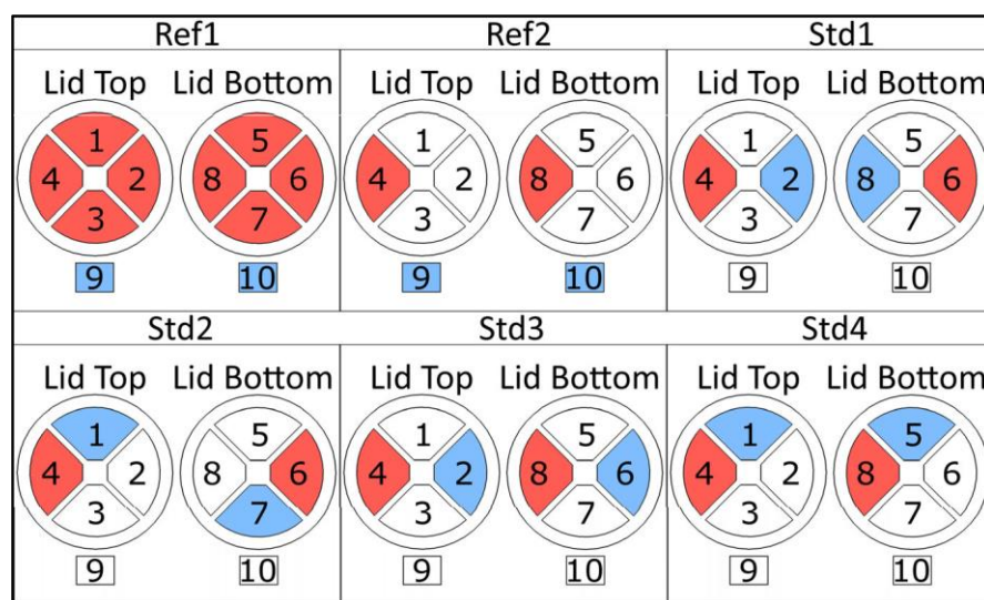
Figure 3 Measured electrode array combinations with red current and blue potential electrodes.
