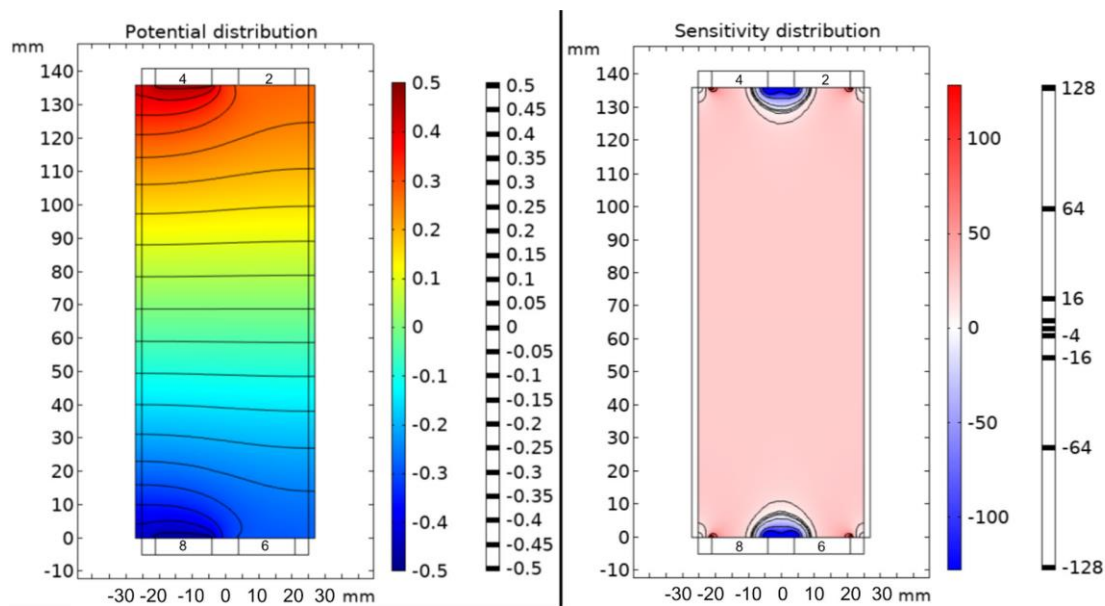
Figure 1 Example of FEM modeling results showing solution for potential field (left) and sensitivity distribution (right) for current and potential electrodes shown in Figure 3; Std3.
