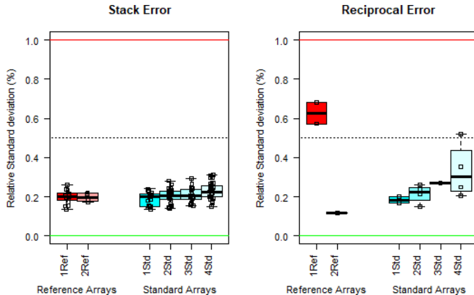
Figure 4 Result of test measurements with sample container filled with tap water. Abbreviations on the x-axis refers to labels in Figure 3
