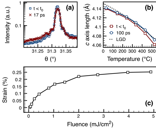
FIG. 4 (color online). Role of depolarization field in photovoltaic response. (a) PTO (003) in the paraelectric phase on DSO at 479 ^\circ\text{C} , slightly above T_C (incident fluence = 5 \text{mJ}/\text{cm}^2 ). Only small \theta shifts are seen due to the centrosymmetric, paraelectric unit cell. (b) LGD theory calculation, comparing the observed c lattice parameter of PTO on STO at t < t_0 and t = 100 ps (incident fluence = 4 \text{mJ}/\text{cm}^2 ) to the predicted zero-field c parameter. (c) Strain in the c parameter of monodomain PTO on STO at 550 ^\circ\text{C} as a function of fluence, measured at t = 100 ps. Saturation behavior in the largest drivable strain is seen.
