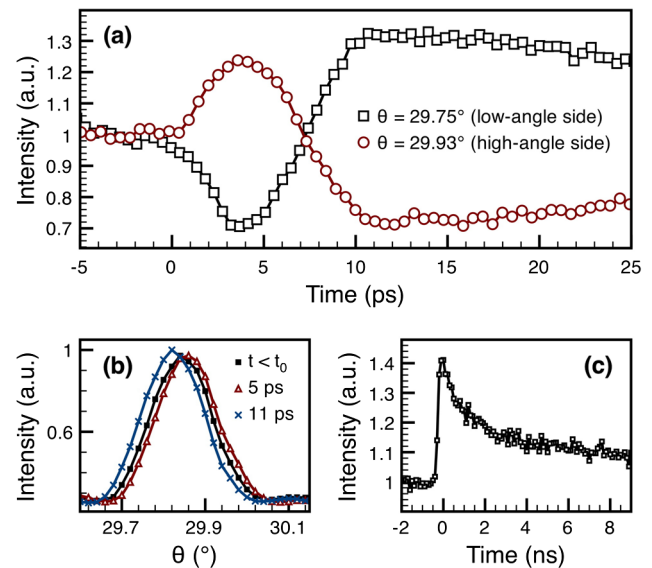
FIG. 1 (color online). Evolution of the tetragonality of PTO in the monodomain phase on STO. (a) Time scans on the low- and high-angle sides of the PTO (003) rocking curve at room temperature (incident fluence = 5 \text{mJ}/\text{cm}^2 ). We observe an acoustically limited high- Q shift, followed by a long-lived low- Q shift. (b) Rocking curve scans at various time delays denoted in (a). (c) Long-range time scan on the low-angle side of PTO (004) at 350 °C (incident fluence = 5 \text{mJ}/\text{cm}^2 ). The observed low- Q shift decays on single-nanosecond time scales.
