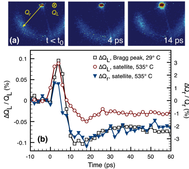
FIG. 2 (color online). Stripe domain phase response at 535 °C. (a) Area detector images of PTO (003) at 535 °C for several time delays (incident fluence = 5 \text{ mJ}/\text{cm}^2 ), corrected such that the angle of the detector plane is normal to the L axis in reciprocal space. (b) Time evolution of Q_L and Q_r , extracted from area detector images of PTO (003). Q_L is the position of the diffuse scattering ring along the L axis and Q_r is the radius of the diffuse ring.
