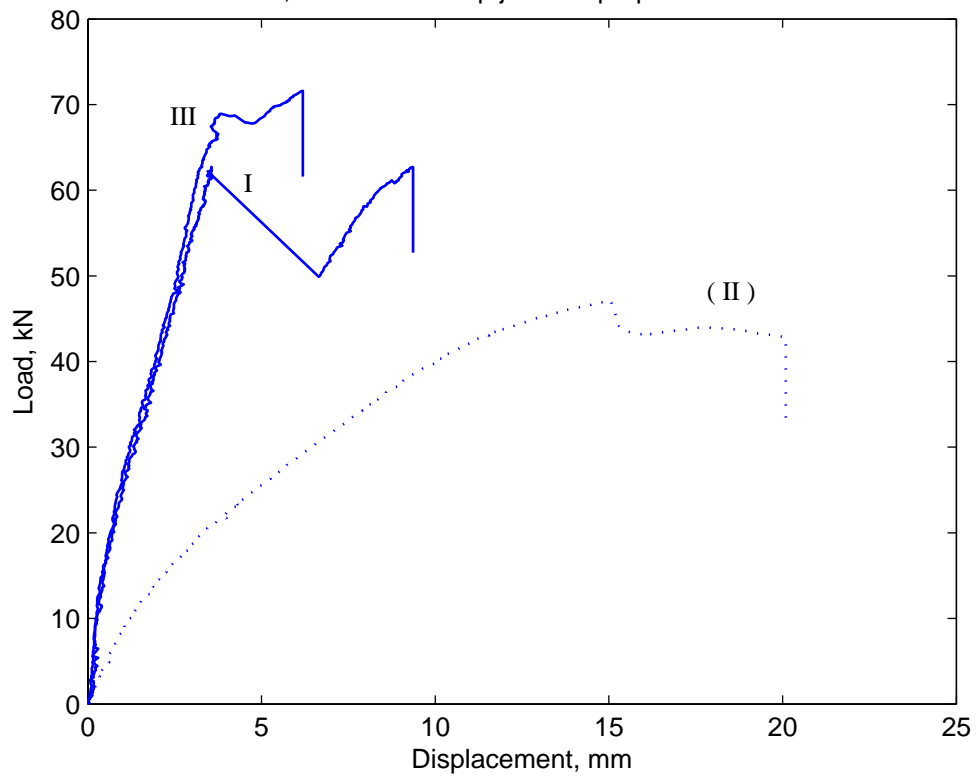
Series 5, 160 mm LVL lap joints in perpendicular tension
