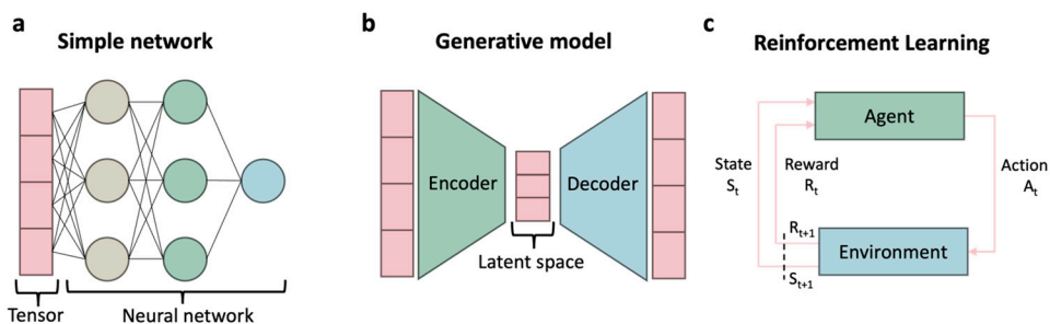
Figure 7: Deep learning models.
