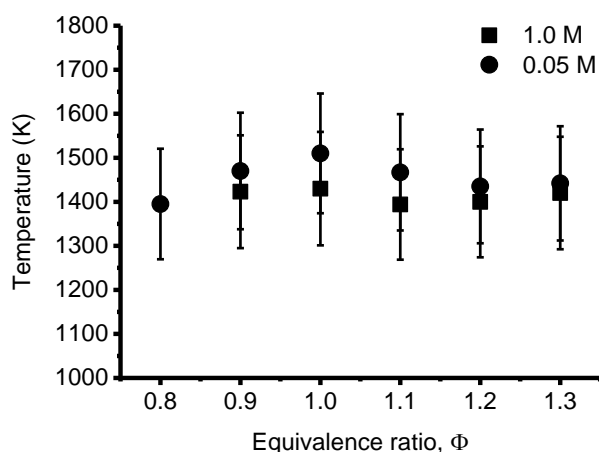
Figure 2. Average temperature in post-flame region of premixed methane-air flames with two different levels of KCl-seeding to the flame. Circles 0.05 M solution, squares 1.0 M solution. The estimated temperature uncertainty is 9% (error bars), the consistently lower temperatures for the 1.0 M case indicate that high levels of alkali salt may induce some cooling.
