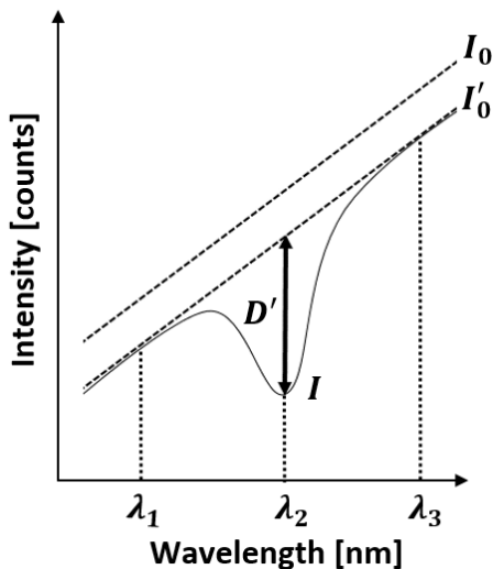
Figure 2.4. Schematic of the spectral evaluation of the DOAS technique where the differential absorbance D' is derived from the fitted low order polynomial I'_0 and transmitted intensity I at resonance wavelength at \lambda_2 .
