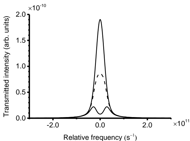
Figure A1. Calculated transmitted intensity for 4^2P K atom emission at negligible absorption (solid single peak), moderate absorption (dashed single peak), and strong absorption, (low dual peak). The strong attenuation at the line center confines emission the wings of the spectral line resulting in a sub-linear dependence on K-atom concentration for the flame chemiluminescence.
