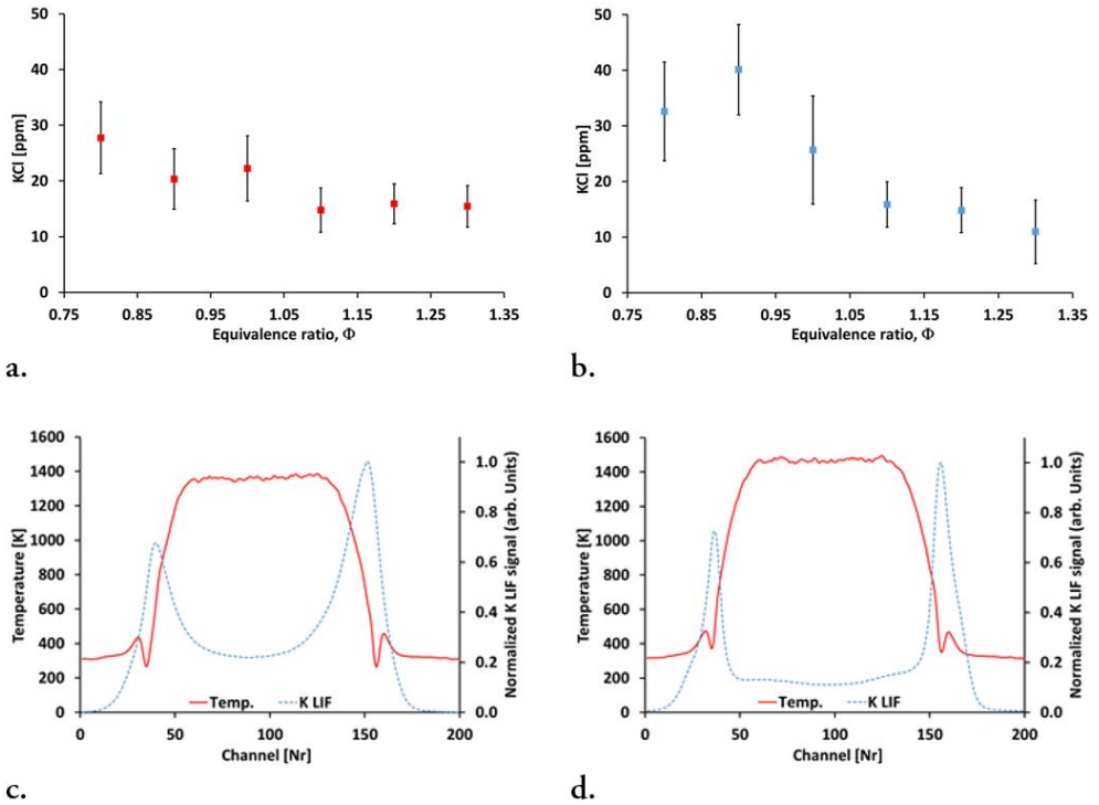
Figure 4.5a. KCl concentrations from absorption measurements at different equivalence ratios measured with the IACM. b. KCl concentration from LI-PFF measurements recalculated to ppm. c. Rayleigh temperature measurement and K LIF signal in a 1 M KCl seeded methane-air flame at \phi = 0.9 . d. Rayleigh temperature measurement and K LIF signal in a 1 M KCl seeded methane-air flame at \phi = 1.3 .
