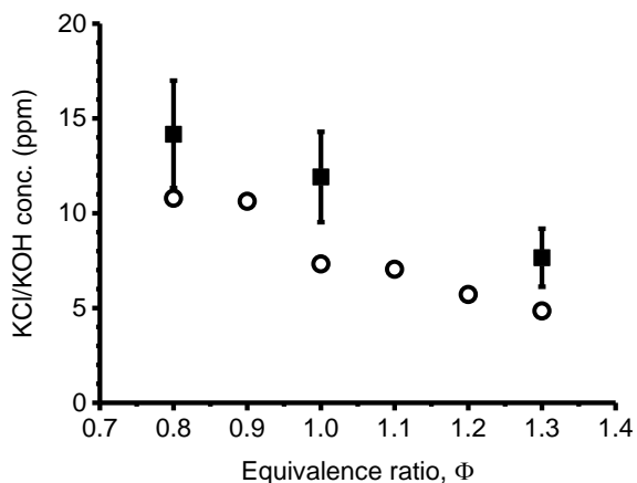
Figure 5. Average post-flame concentration versus flame equivalence ratio measured using laser-induced photofragmentation fluorescence for seeding of a) 0.5 M KOH and b) 0.5 M KCl. Lower KOH/KCl concentrations are measured at fuel-rich conditions due to increased formation of K atoms. Circle symbols represents results from calculations of potassium species concentrations a) KOH and b) the sum KCl+40% KOH.
