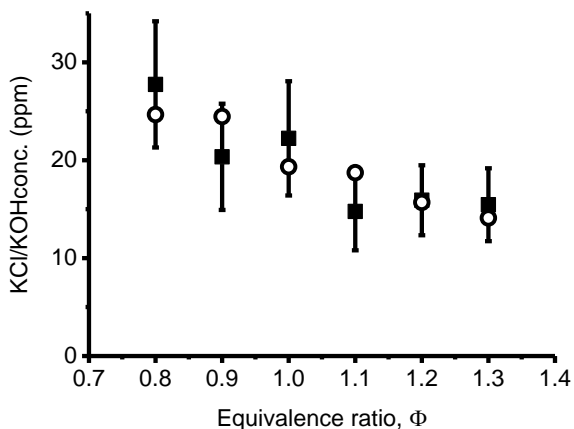
Figure 4. Average post-flame concentration measured by UV absorption spectroscopy versus flame equivalence ratio for 1.0 M KCl seeding. Lean conditions show higher KCl concentrations. Circle symbols represents the sum KCl+50% KOH of calculated potassium species concentrations.
