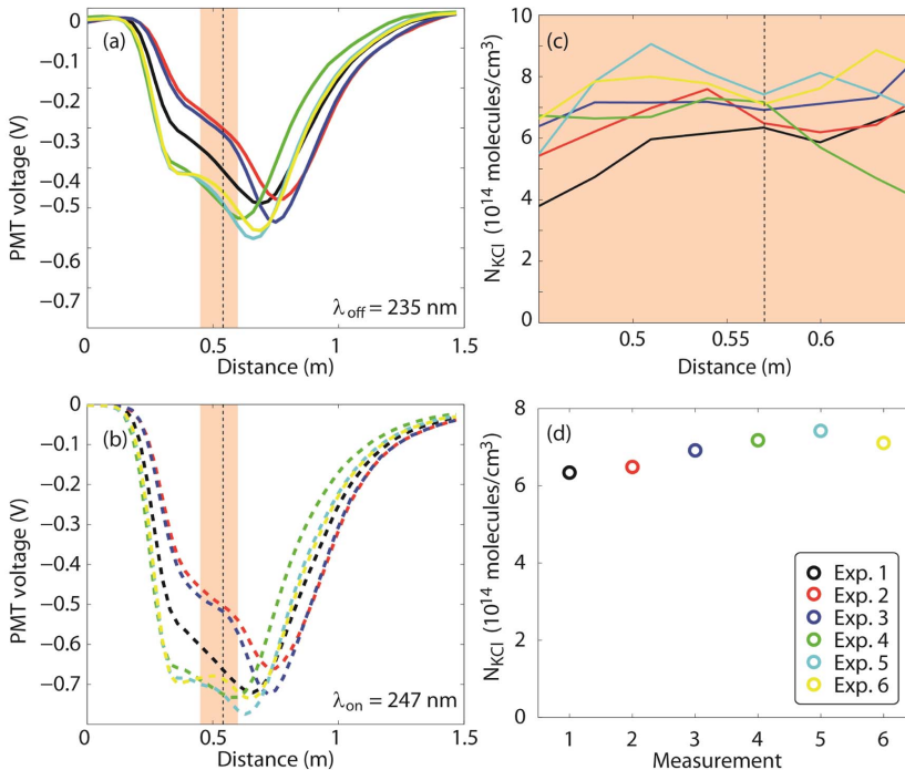
Fig. 6. Double-pulse ps-DIAL data, each signal consists of 100 single shots and each pair is displayed in different color coding. Raw-data of the back-scattered signal from (a) 235 nm and (b) 247 nm. (c) Range-resolved concentration data of KCl inside the tube furnace. The range is indicated with a colored area in (a) and (b). (d) Number densities evaluated for the six signal pairs at distance 0.57 m, indicated by a dashed line in (a), (b), and (c).
