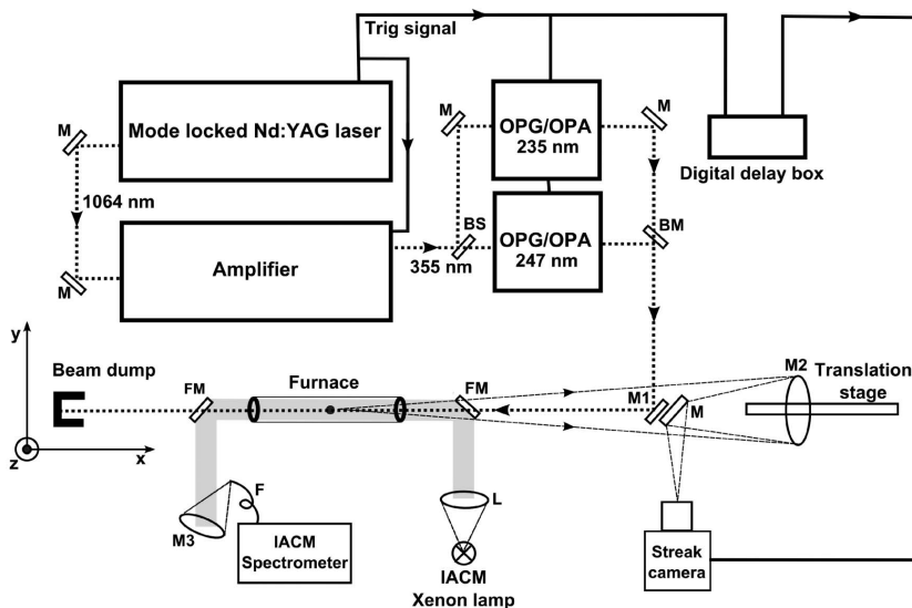
Fig. 1. Experimental setup for combined DIAL and IACM measurements on vaporized KCl . M designate planar mirrors, BS a beam splitter, and BM a beam combining mirror. The laser beams are guided into the furnace by mirror M1 and backscattered laser light is collected with concave spherical mirror M2. For IACM, L is a plano-convex lens for collimation of the Xenon lamp light (gray), FM indicates flip-in mirrors, and M3 is a concave spherical collection mirror.
