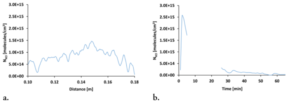
Figure 4.1a. Shows the KCl number density calculated with the simplified DIAL equation Eq. (2-10). b. Shows the KCl concentration before and after the DIAL measurements.
