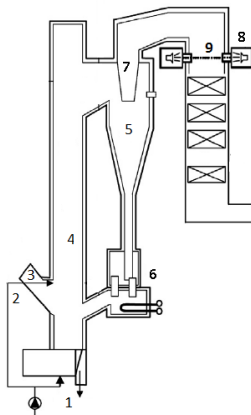
Figure 1a. Principle sketch of the Circulating Fluidized Bed (CFB) boiler with its key components listed below. 1. Primary air 2. Secondary air 3. Fuel feeding 4. Furnace 5. Cyclone 6. Particle seal 7. Cyclone outlet 8. IACM and 9. Measurement path length.
