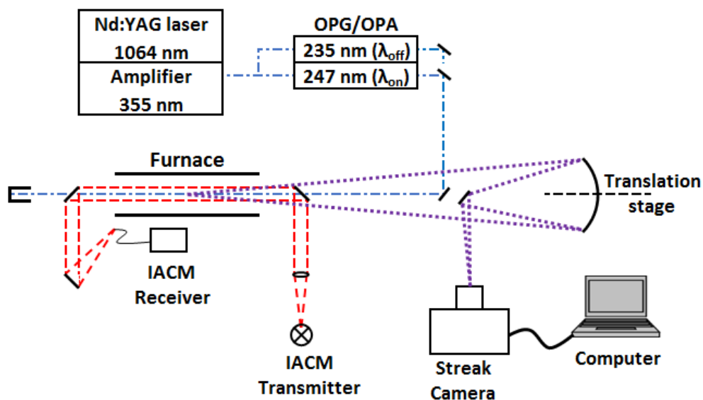
Figure 3.1. The experimental set-up for DIAL and IACM measurements used in Paper I. The blue (dashed dot) line indicates the beam path for the 235 nm \lambda_{off} and the 247 nm \lambda_{on} off and on KCl resonance, respectively used during the DIAL measurements. The red (dashed) line shows the beam path for the KCl measurements with the IACM instrument. The purple (dotted) line shows the backscattered light used to determine the KCl concentration by means of DIAL measurements.
