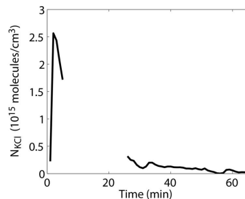
Fig. 5. KCl concentration profile monitored by IACM before and after the ps-DIAL measurements carried out during the time interval where the curve is broken.
