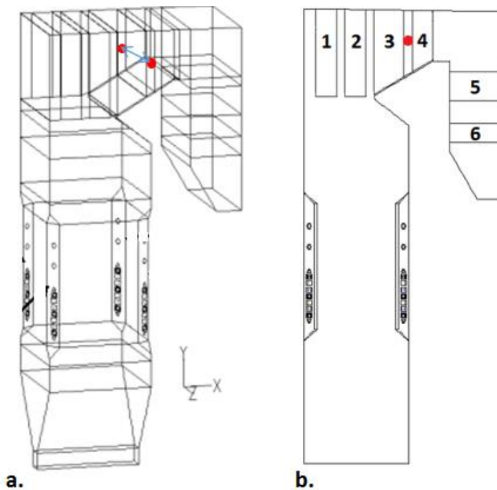
Figure 3.11a. A drawing of the PF boiler with a furnace width in x-direction of 7.6 m and a depth in z-direction of 8.1 m. b. The IACM is situated between superheaters 3 and 4. The location is marked with two red dots and the measurement path length is 8 m.
