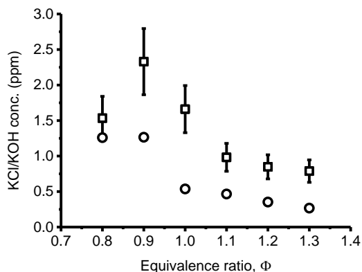
Figure 6. KCl/KOH concentration versus flame equivalence ratio measured using laser-induced photofragmentation fluorescence for seeding with different potassium and chlorine levels. a) 1.0 M KCl seeding b) 0.05 M KCl seeding. Lower KCl/KOH concentrations are obtained under fuel-rich conditions. Circle symbols represents results from calculations of potassium species concentrations a) the sum KCl+40% KOH and b) KOH.
