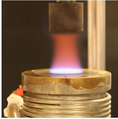
Figure 1. Methane-air flame of equivalence ratio \Phi=1.1 stabilized on porous plug Perkin-Elmer burner with alkali-seeding (KCl) through a nebulizer. Laminar uniform flames were achieved with a stabilizer mounted 30 mm above the burner surface.
