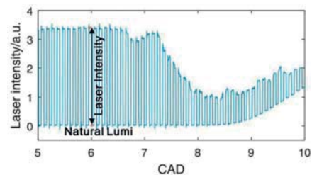
Figure 3. Raw data from photodiode (transmitting)
