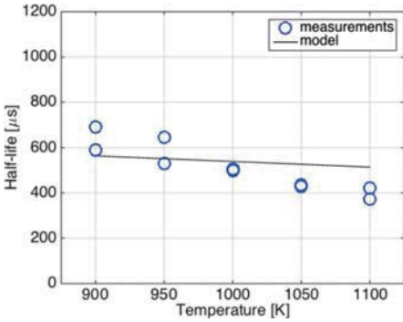
Figure 7 (b). Half-lives for a sweep of temperature at TDC
