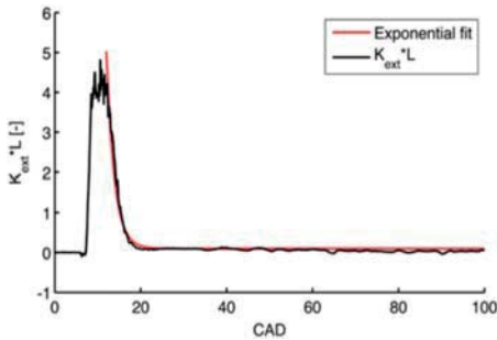
Figure 9b. Ensemble average over 29 K_{ext}L curves for the 21% O_2 case and exponential decay fit.
