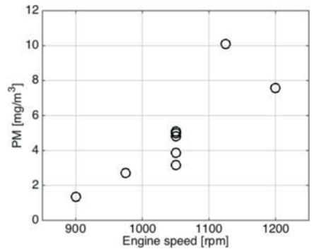
Figure 4 (d). Exhaust PM levels for a sweep of engine speed.
