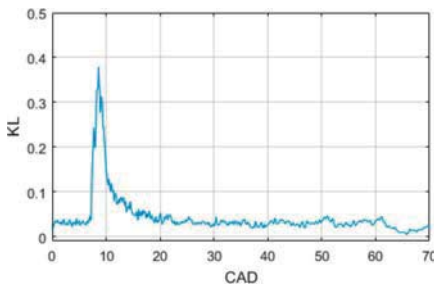
Figure 9. KL curve in the no combustion case.
