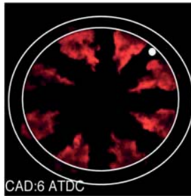
Figure 5. Combustion pattern at 6 CAD ATDC. Natural luminosity of soot was recorded. The white area represents the position of the laser during the measurements. The inner white circle represents the bowl wall; the outer one represents the periphery of the piston.
