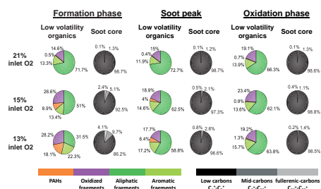
322 Figure 3: Soot chemical compositions during soot formation, soot peak and soot oxidation phases 323 for 21%, 15% and 13% inlet O 2 concentrations. Left columns: grouped ion fragments originating
