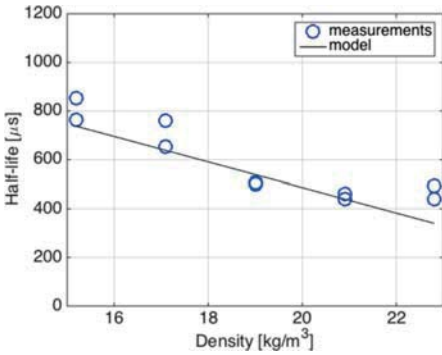
Figure 7 (a). Half-lives for a sweep of density at TDC
