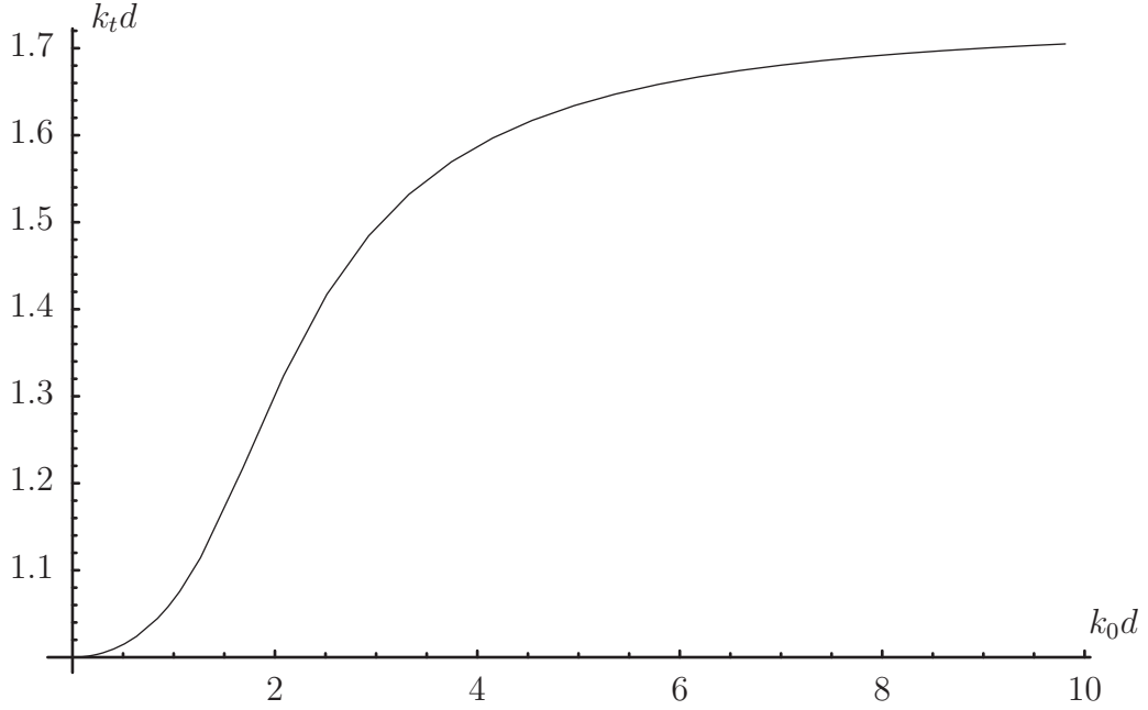
Figure 6: The normalized wave number k_t d of the surface wave as a function of the normalized frequency k_0 d of the \text{TM}_0 -mode for an isotropic profile \epsilon = 3 and \mu = 1 .
