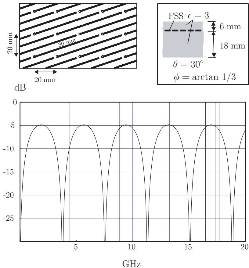
Figure 16: The reflection coefficient for the perpendicular polarization (TE-case) for an array of gangbuster elements (type 3) that supports several surface waves in the frequency interval depicted. The onset of the first two grating lobes occurs at 10.25 GHz ( m = -1, n = 0 ) and 14.43 GHz ( m = 0, n = -1 ), and the onset of the first two non-zero surface wave ( TE_1 and TM_1 ) occurs at 4.42 GHz and 8.83 GHz, respectively. Note that the surface waves are not excited in this case.
