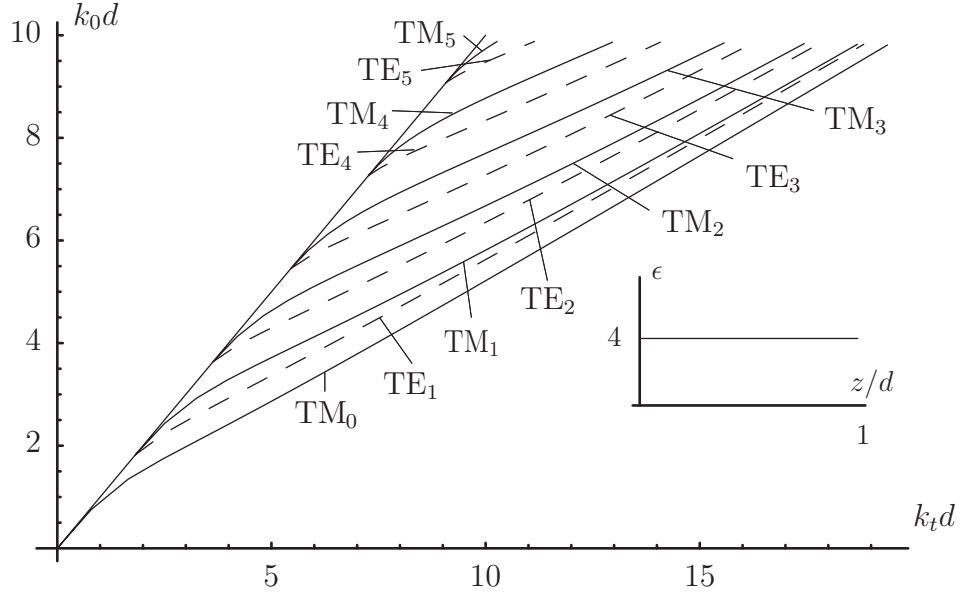
Figure 4: The normalized frequency k_0 d = \omega d/c_0 as a function of the normalized wave number k_t d of the surface mode. The figure shows the dispersion curves for an isotropic profile \epsilon = 4 and \mu = 1 . The k_0 d -values for the onset of the different modes for the profile are: TE_1 = TM_1 = 1.81 , TE_2 = TM_2 = 3.63 , TE_3 = TM_3 = 5.44 , TE_4 = TM_4 = 7.26 , and TE_5 = TM_5 = 9.07 . The solid lines show the TM-modes and the dashed lines the TE-modes.
