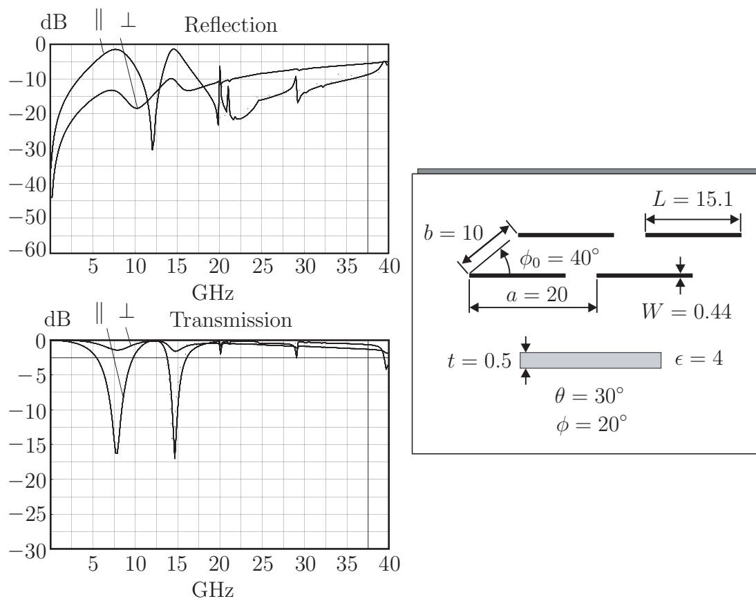
Figure 10: The reflection and transmission coefficients, i.e. , the radiated power in the k_{t00} direction, for a skewed array of dipoles in the parallel (TE) and the perpendicular (TM) polarizations. The onset of the two first grating lobes occurs at 21.27 GHz ( m = -2, n = -1 ) and 22.13 GHz ( m = -1, n = 0 ), and the onset of the first non-zero surface wave ( TE_1 ) occurs at 173 GHz. In Figure 11, the frequency interval between 19–24 GHz is shown in detail.
