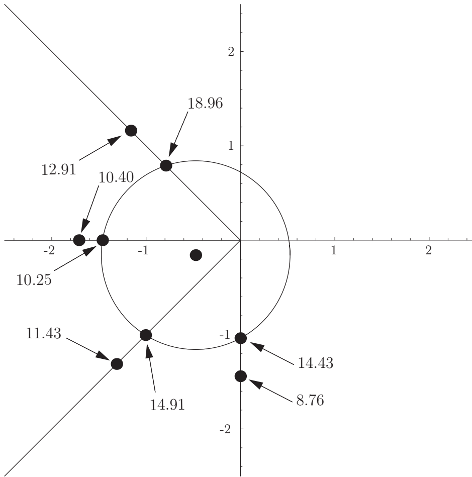
Figure 14: The geometrical interpretation of the onset of the grating lobes and the excitation of the surface waves for a \text{TM}_1 -mode in Figure 12. The solid dot in the center of the circle marks the direction of the incident field, i.e. , (u_i, v_i) .
