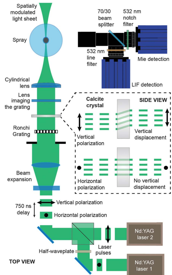
Fig. 1. Top view of the optical arrangement of 2p-SLIPI setup for simultaneous LIF and Mie detection. A spatially modulated light sheet is created by means of a Ronchi grating, while the displacement of the line pattern is operated by employing the birefringence of a calcite crystal, as illustrated in the zoomed area.
