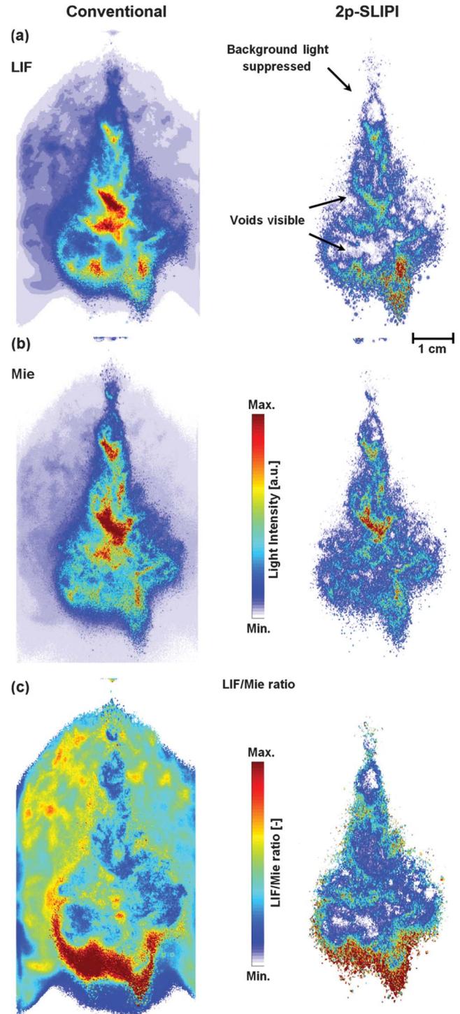
Fig. 3. Comparison between conventional light sheet imaging and 2p-SLIPI for instantaneous (a) LIF, (b) Mie scattering, and (c) LIF/Mie ratio. The transient ethanol spray is imaged at 2500 \mu s after the visible start of the injection. The 2p-SLIPI approach generates images cleaned up from multiple scattering artifacts.
