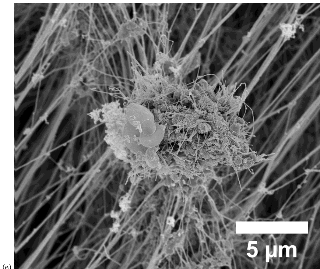
Fig. 3. SEM images of airborne agglomerates of MWCNTs collected in the breathing zone of the worker in the production laboratory with a Sioutas Personal Cascade Impactor. Typical particles from the different stages are presented. Soot aggregates present in the MWCNT powder as an impurity can also be seen in the SEM images. a) MWCNT-containing particles collected at the stage > 2.5 \mu\text{m} . b) MWCNT-containing particles collected at the stage 2.5\text{-}1.0 \mu\text{m} . c) MWCNT-containing particles and carbon nanodiscs collected at the stage 1.0\text{-}0.50 \mu\text{m} . d) MWCNT-containing particles and carbon nanodiscs collected at the stage 0.50\text{-}0.25 \mu\text{m} . e) Carbon nanodiscs collected on the after filter ( < 0.25 \mu\text{m} ) made of polytetrafluoroethylene (PTFE, Teflon). An airborne agglomerated MWCNT particle is also visible in the image.
