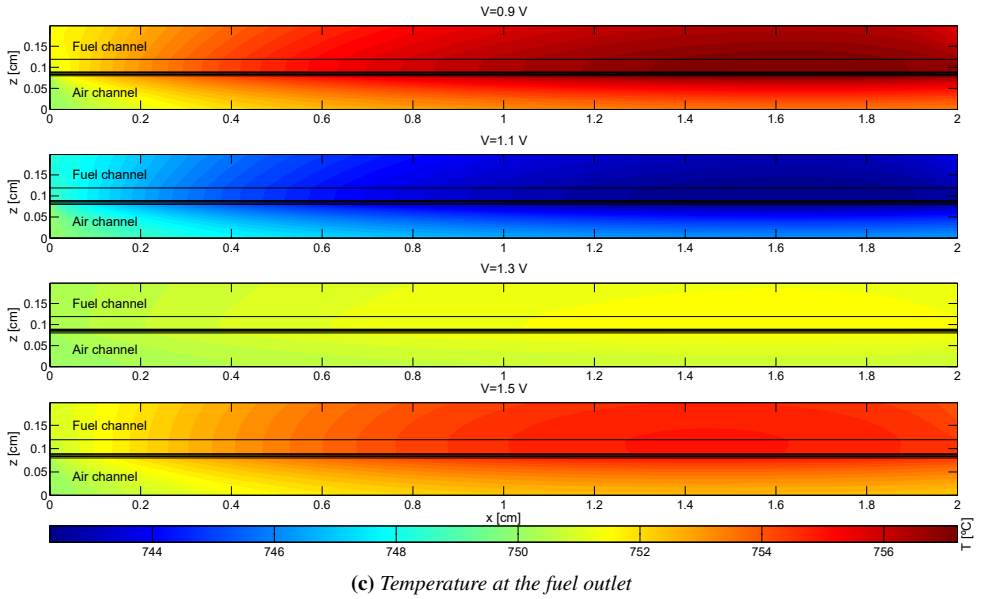
Figure 9: p_{\text{H}_2\text{O}} profile along the fuel direction, overpotential distribution through the cell and temperature distribution at the fuel outlet for four different cell voltages at p_{\text{H}_2\text{O}} = 0.5 atm and 750^{\circ}\text{C} .
