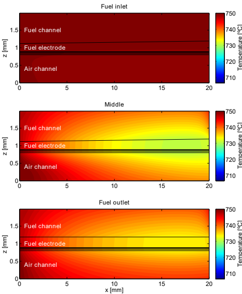
(c) T with heat flux boundary condition
