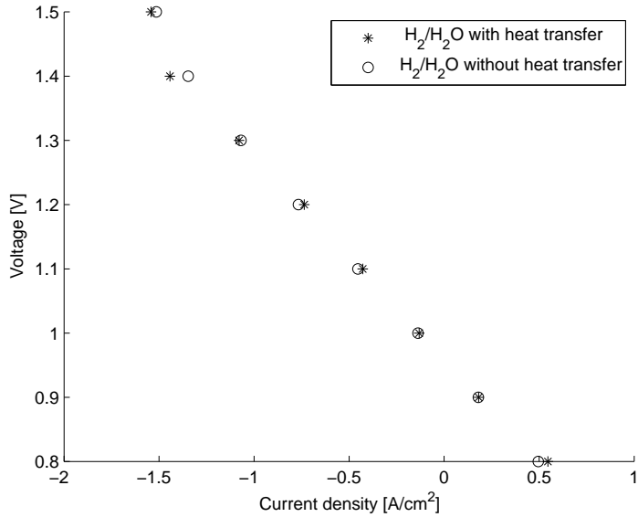
Figure 10: Comparison of i - V curves with and without heat transfer at p_{\text{H}_2\text{O}} = 0.5 atm and 750\text{ }^\circ\text{C} .
