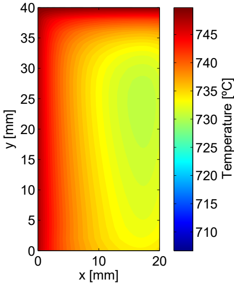
(a) T with heat flux boundary condition
