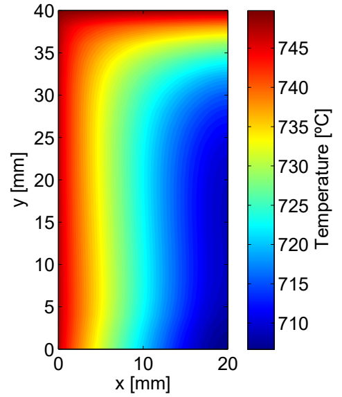
(b) T with thermal insulation
