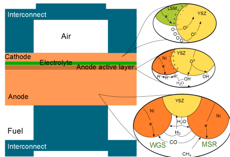
Figure 1. Schematic image of an SOFC with some detail on surface chemistry.
