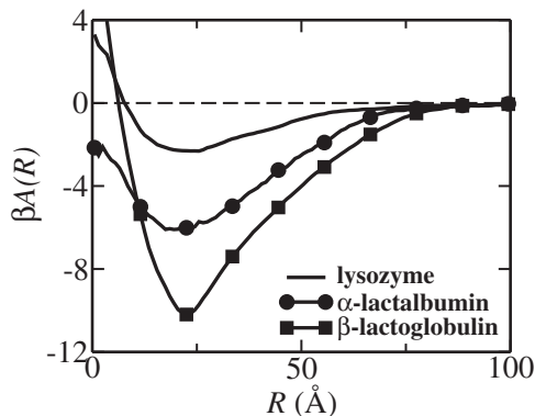
Fig. 8. The free energy of interaction between the centers of mass of the protein and the polyelectrolyte at low salt concentration obtained from MC simulations with model B (da Silva et al. 2006). The curves have been calculated at the respective isoelectric points for lysozyme (no symbols), \alpha -lactalbumin (filled circles) and \beta -lactoglobulin (filled squares).
