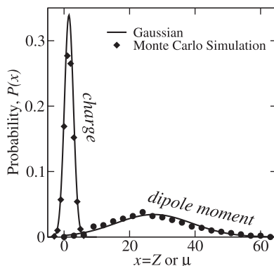
Fig. 10. Probability function for the net charge, Z and dipole moment \mu of the protein hisactophilin at pH 7. The symbols represent the sampled histograms from a Monte Carlo simulation of the protein in a salt solution while the solid lines are Gaussians plotted from the averages and variances.
