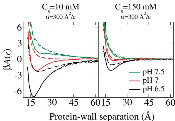
Fig. 6. Free energy of interaction of hisactophilin with a negatively charged surface at various pH and salt concentrations, C_s . Calculated using coarse-grained Monte Carlo simulations with (full drawn lines) and without (dashed lines) charge regulation and with a surface area per charge of 300 \text{ \AA}^2/e . (Lund et al. 2005)
