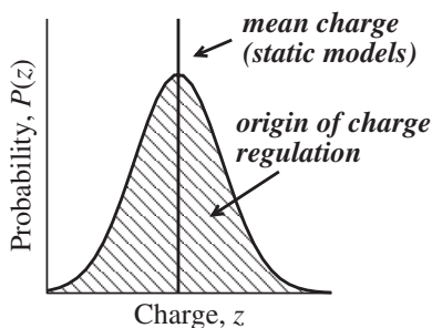
Fig. 1. In addition to the average charge, \langle z \rangle , a titratable site also has a variance, \epsilon , around the mean. The distribution – often well described by a normal distribution – is the origin of the charge regulation mechanism.
