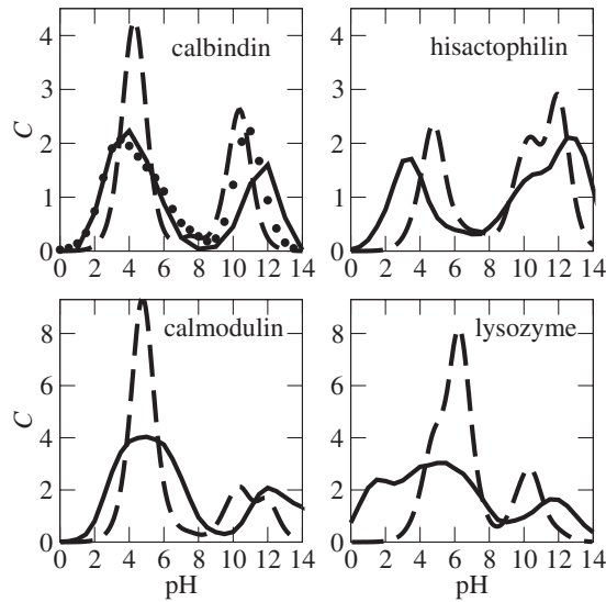
Fig. 2. Capacitances, C , as a function of pH for four different proteins in aqueous solutions with 30 mM 1:1 salt. Shown for simulated (fully drawn), ideal (dashed) and experimental data where available (symbols).
