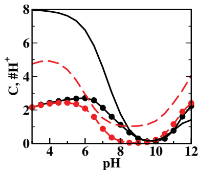
Fig. 5. Number of protons, \#H^+ , released in calmodulin (CaM) upon binding of four calcium ions (black solid line) and upon binding a heptavalent peptide (dashed red line) as a function of pH. The black solid line with symbols shows the capacitance, C , for CaM without calcium ions and red dashed line with symbols shows the capacitance for CaM with four calcium ions bound.
