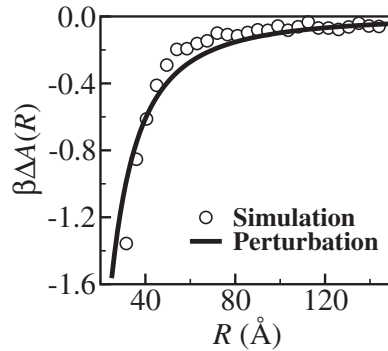
Fig. 4. The difference in free energy of interaction between calbindin and lysozyme at pH 4 for a protein model with regulation and one with fixed charges. R is the separation between the mass centra of the two proteins and symbols denote the simulated difference and the solid line is obtained from Eq. (15) with Z_{\text{calb}}=1.16 , C_{\text{calb}}=2.23 , Z_{\text{lys}}=10.2 and C_{\text{lys}}=0.88 .
