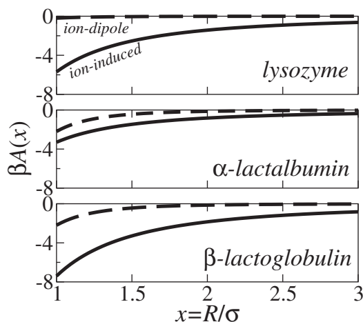
Fig. 7. Ion-induced charge (solid lines) and ion–dipole (dashed lines) contributions to the free energy of interaction between a polyanion and three different proteins. Calculated from Eq. (15) augmented with an ion–dipole term using simulated capacitances and dipole moments (da Silva et al. 2006).
