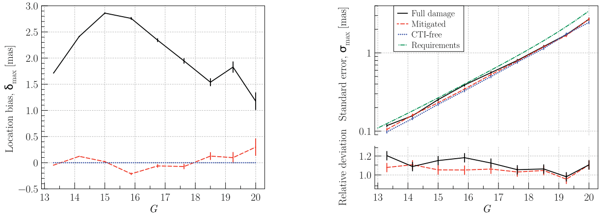
Figure 3. \delta_{\max} and \sigma_{\max} in the ‘full-damage’ (black continuous line) and ‘mitigated’ (red dashed line) cases (see Section 2.2.2) as obtained in Paper I for the Gaia operating conditions, the ‘typical’ profile width and an active trap density of 1 trap pixel -1 (see, in Paper I, figs 12 and 13 for the damaged case, figs 20 and 21 for the mitigated case and fig. 10 for the standard error of the CTI-free case, and tables 1 and 2 for biases and standard errors). These values are used to construct our CTI model, shown in Fig. 6. Left: \delta_{\max} , maximum image location bias in mas as a function of magnitude ( G band) induced by CTI effects with (red dashed line) and without (black continuous line) applying a CTI mitigation procedure. The error bars correspond to the statistical uncertainties. Right: \sigma_{\max} , maximum image location standard errors in mas as a function of G induced by CTI effects with (red dashed line) and without (black continuous line) applying a CTI mitigation procedure. The Gaia requirements (green dot-dashed line) for a single CCD transit and the CTI-free case (blue dotted line) are also shown. The relative deviation from the later is computed (bottom panel) for the ‘full-damage’ case (black continuous line) and the ‘mitigated’ case (red dashed line).
