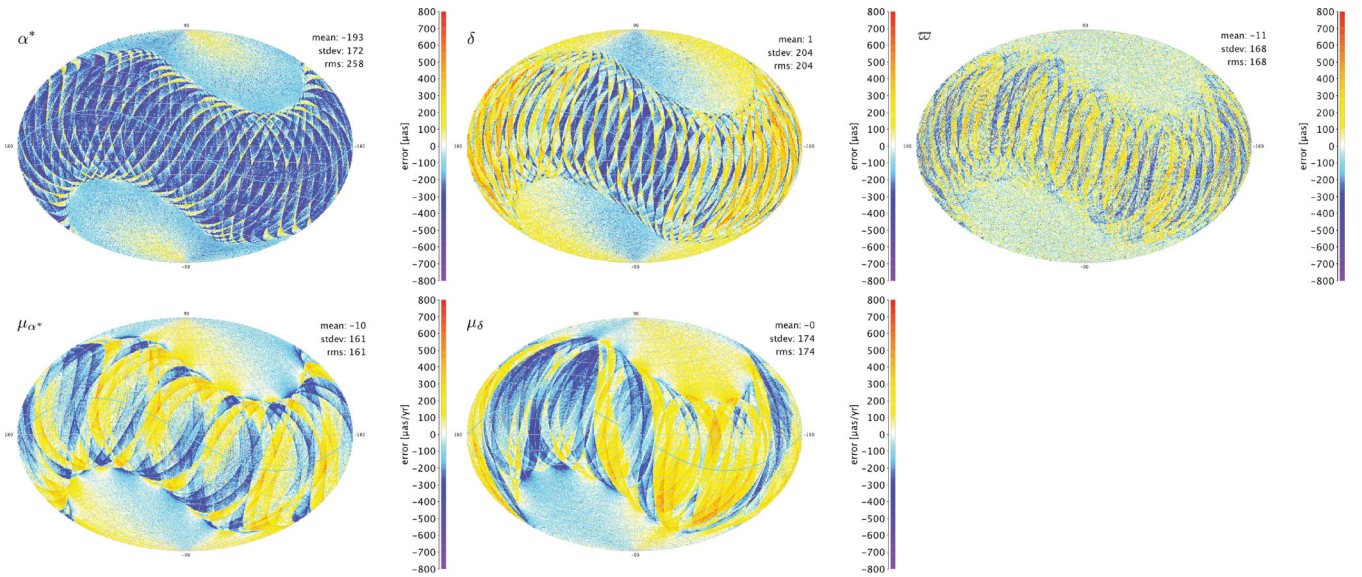
Figure 8. Errors in position ( \alpha^* , \delta ), parallax ( \varpi ) and proper motion ( \mu_{\alpha^*} , \mu_{\delta} ) produced by a constant AL bias of 1000 \mu\text{s} (1 mas). See Section 3.1 for a detailed discussion of these plots.
