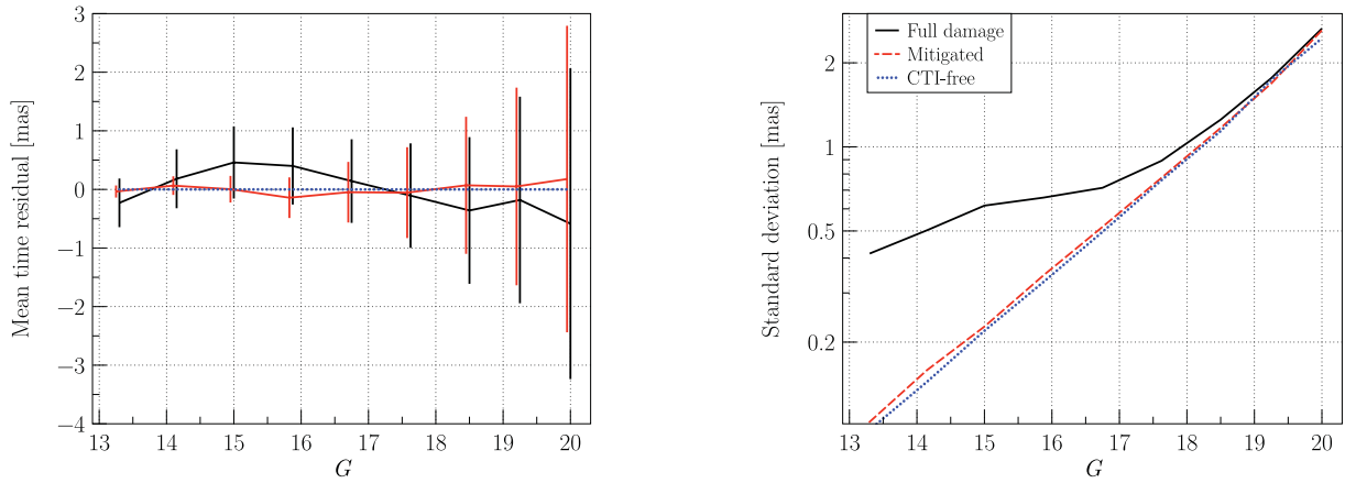
Figure 9. Mean values (left) and standard deviations (right) of the AL residuals in the astrometric solution for all the observations as functions of G . The curves are for the full-damage (solid), mitigated (dashed) and CTI-free (dotted) cases. These diagrams can be directly compared with the applied errors in Fig. 6. Note how the residuals are shifted down, with respect to the applied errors, so that the weighted mean bias is 0. The standard deviation necessarily includes the large residual fluctuation with mission time and time since CI (left-hand plot in Fig. 10), and can therefore not be directly compared with the standard deviations shown in the right-hand plot of Fig. 10.
