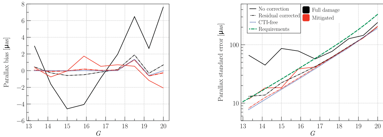
Figure 17. Mean parallax error (left) and standard error (right) per magnitude, with and without the residual correction described in Section 3.3.
