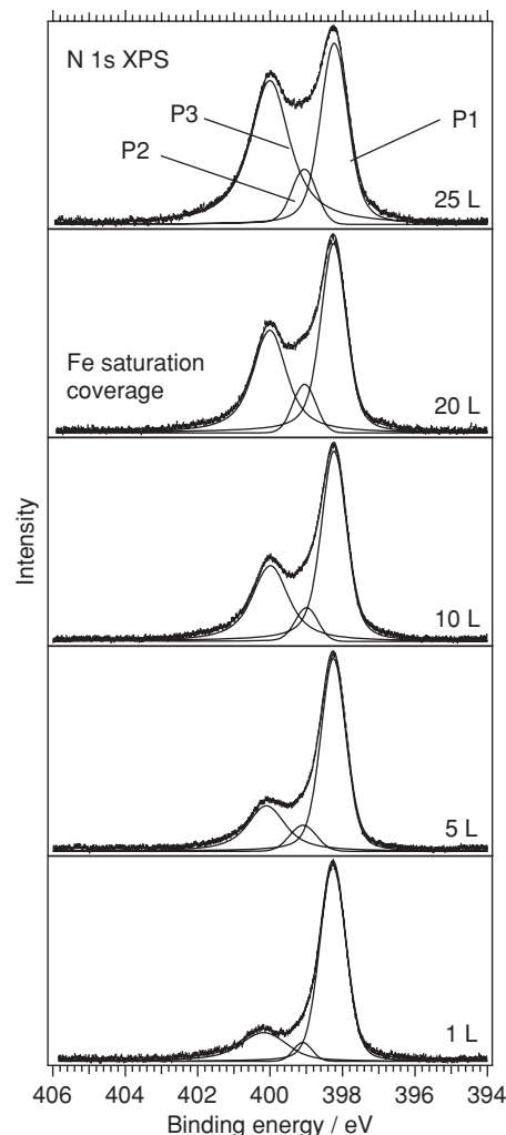
FIG. 8. N 1 s photoelectron spectra (experimental data and fits) for the adsorption of 1–25 L of ammonia on one monolayer of FePc on Au(111). The results show several peak components, P1 due to FePc nitrogen, P2 due to ammonia molecules interacting with the gold (Au–NH 3 bond), and P3 related to the ammonia molecules in different sites.
