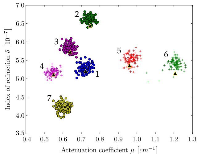
Fig. 2. The scatter plot displays the attenuation coefficient and refractive index decrement for all pixels in the 10 \times 10 \text{ pixel}^2 ROIs in the fluid phantom reconstructions (cf. figure 1, (b) and (c)). Black triangles are the calculated values. Most substances show an overlap in either attenuation or phase signal alone, but all substances can clearly be distinguished using the combined information from both attenuation and phase. The different data clusters are labeled by numbers as used in tables 1 and S1.
