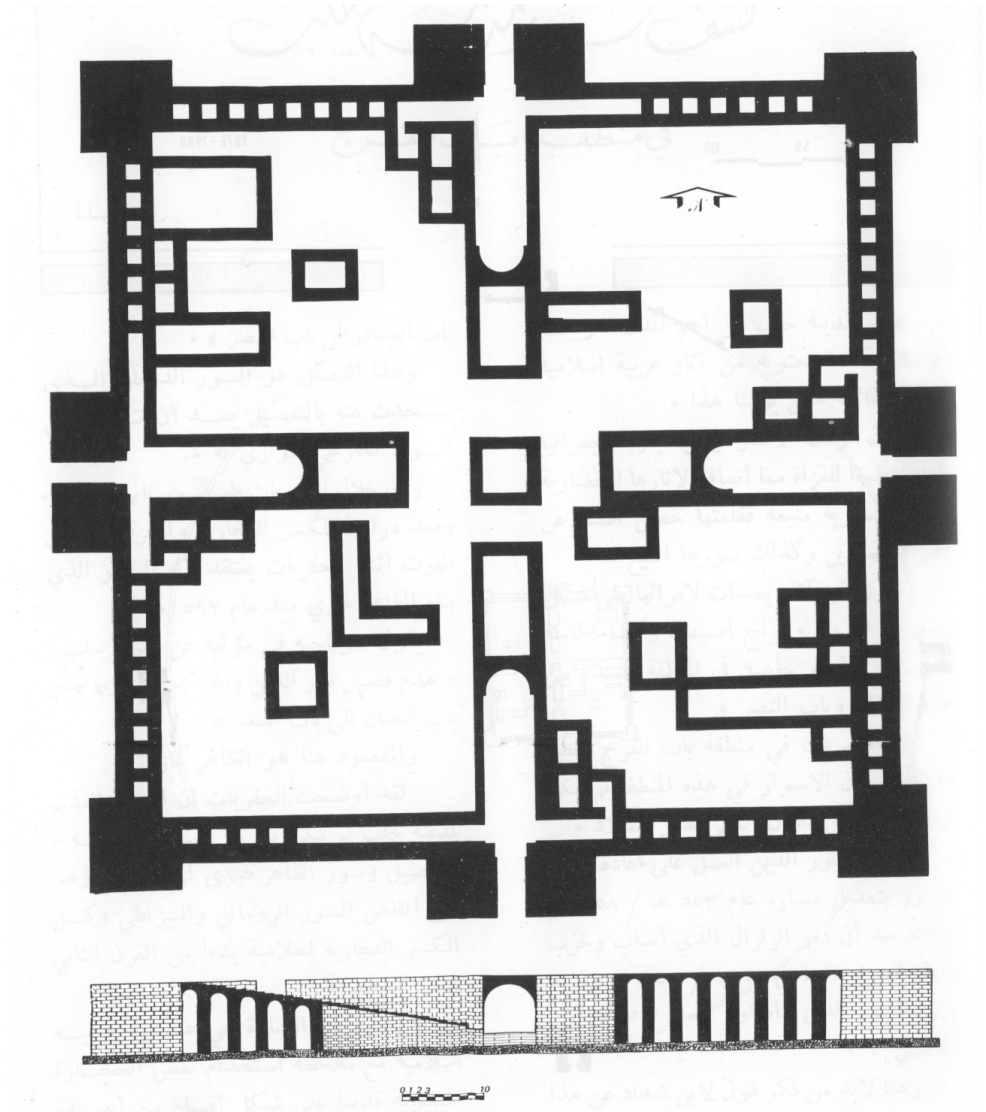
Fig. 10: Plan of the central building (after Touyr, 1983: 111).
