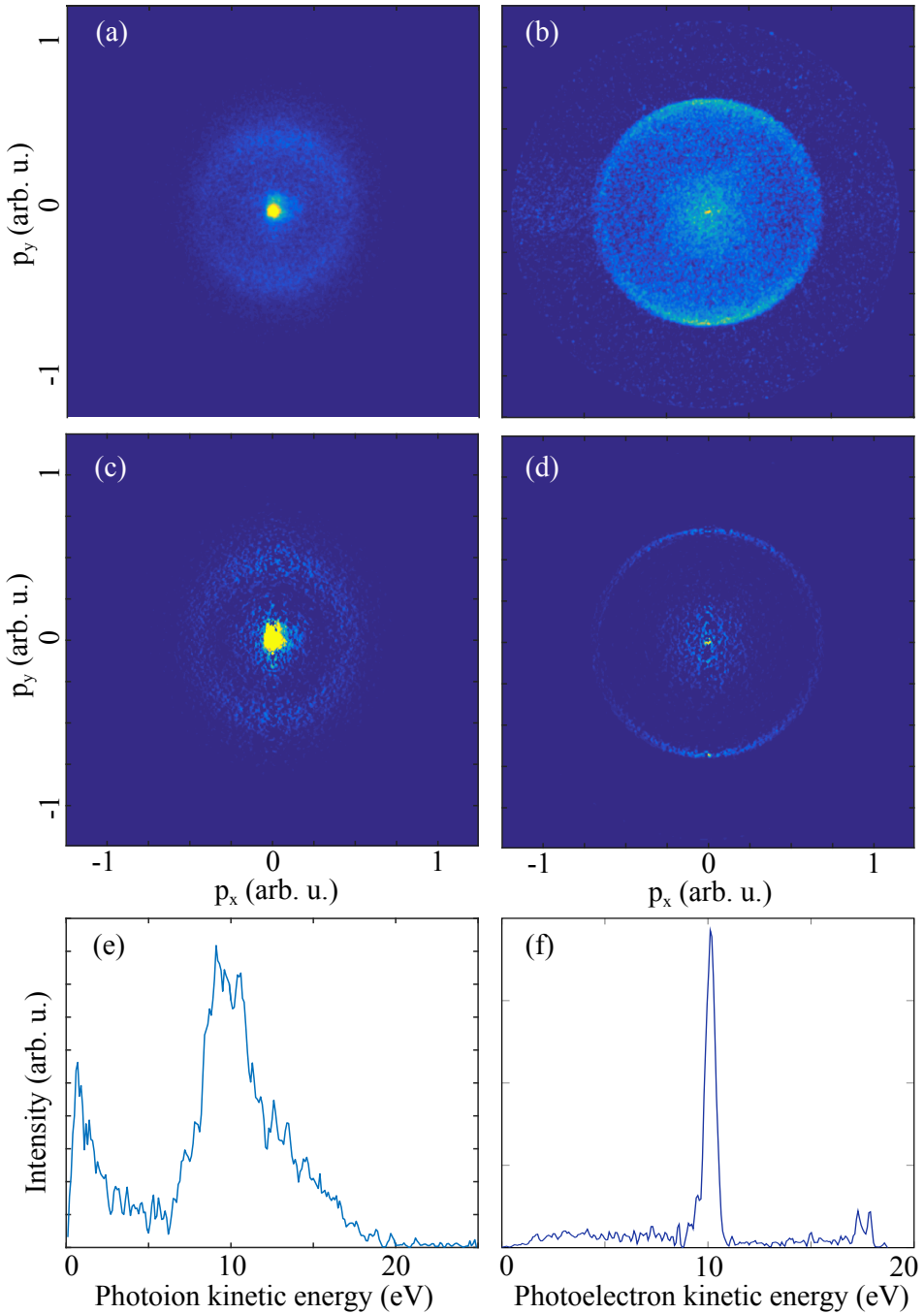
Figure 3.6: Raw (panel (a) and (b)) and inverted images (panel (c) and (d)) from the DVMIS when N_2 is ionized with photons with E_{\text{ph}} = 420 eV. The ions resulting from Coulomb explosion are seen in the left column and electrons with energy of E_{\text{ph}} - Ip are seen in the right column. Panel (e) and (f) show the photoion and photoelectron spectrum, respectively.
