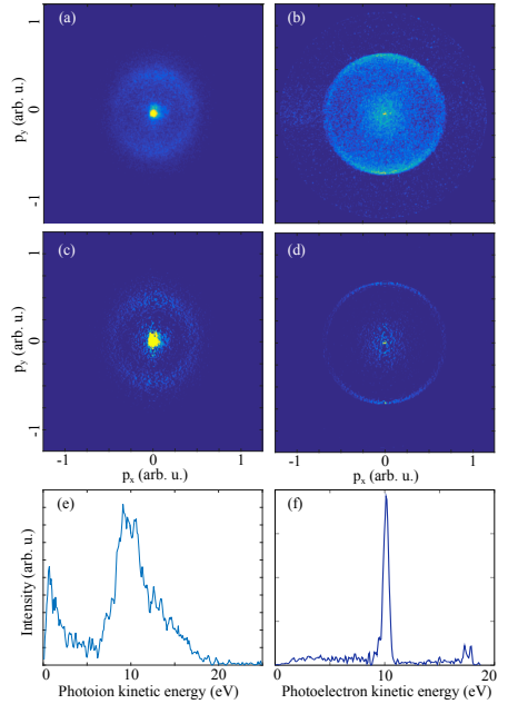
FIG. 7. Experimental results from ionization of \text{N}_2 using 420 eV photons at Max-lab beamline I1011. The measured detector images for photons (a) and -electrons (b) are shown together with the corresponding 3D momentum distributions [(c) and (d)] obtained through inversion. Panels (e) and (f) show the photoion and -electron kinetic energy spectra calculated from the 3D momentum distributions.
