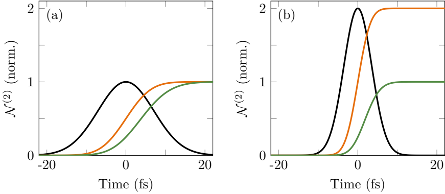
Figure 2.7: Yields of doubly charged ions for the sequential process (green) and the direct process (orange) for a Gaussian pulse (black), for a pulse length of (a) 20 fs and (b) 10 fs. The final yield of the doubly charged ion for the SP is not dependent on the pulse duration and is the same in (a) and in (b) while the final yield of doubly charged ions for the direct process is doubled in (b).
