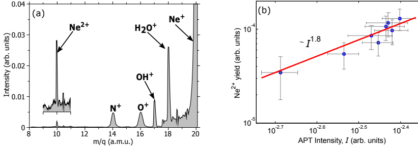
Figure 4.13: Two-photon double ionization of Neon. (a) A mass spectrum from the ion TOF showing the \text{Ne}^{2+} peak at m/q = 10 . (b) The \text{Ne}^{2+} yield as a function of the intensity of the attosecond pulse train. The slope is close to two when using logarithmic scales. Reproduced from Paper III
