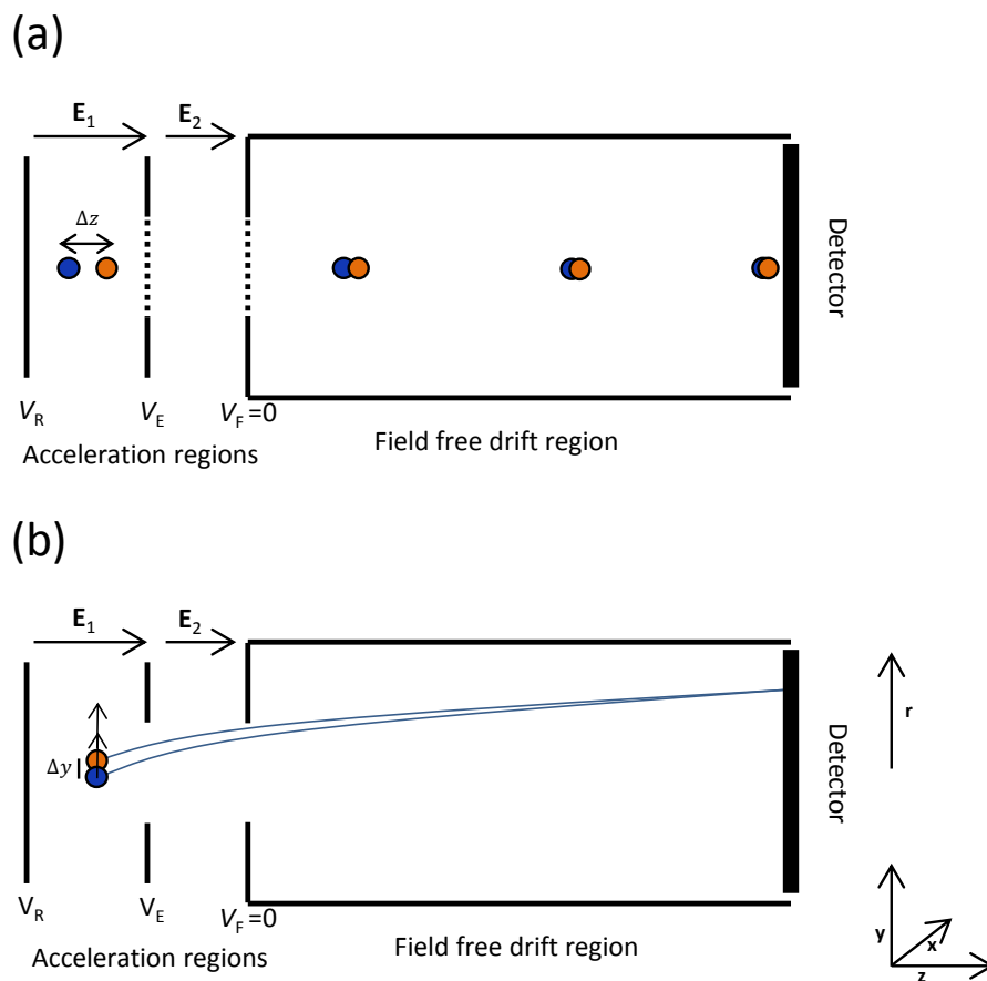
Figure 3.2: (a) An ion TOF operated in Wiley-McLaren conditions where two fragments generated at different positions arrive at the same time at the detector. By tuning V_E the distance where the blue particle catch up with the orange is changed. (b) A VMIS where the position on the detector depends only on the initial momentum in the xy -plane and not on the starting position along the y -axis. By tuning V_E the curvature, and therefore the acceleration in the xy -plane, is adjusted to compensate for the initial spread of the starting positions.
