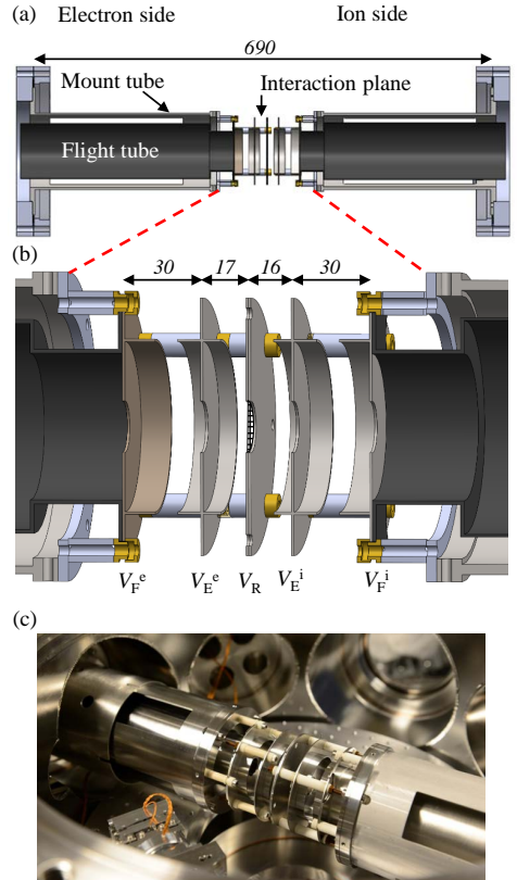
FIG. 2. Drawing of the double VMIS (a) and an expanded view of the electrode package (b). The indicated voltages are applied to the electron side flight tube ( V_F^e ), the electron side extractor ( V_E^e ), the repeller ( V_R ), the ion side extractor ( V_E^i ) and the ion side flight tube ( V_F^i ). A photo of the spectrometer mounted in the experimental chamber is shown in panel (c).
