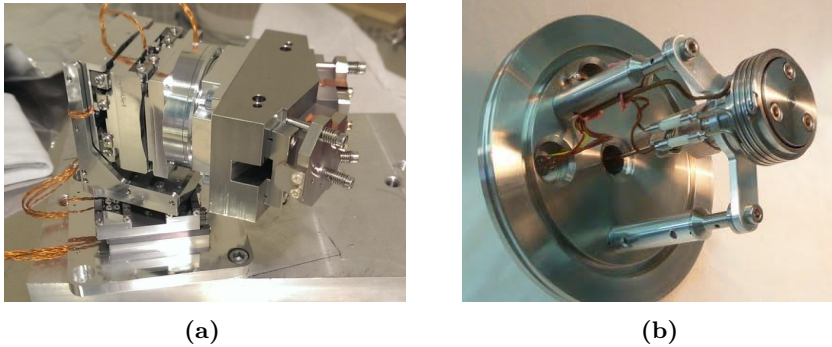
Figure 4.7: (a) Focusing optics mounted in a five-axis mount, and (b) the Even-Lavie valve mounted on a flange.
