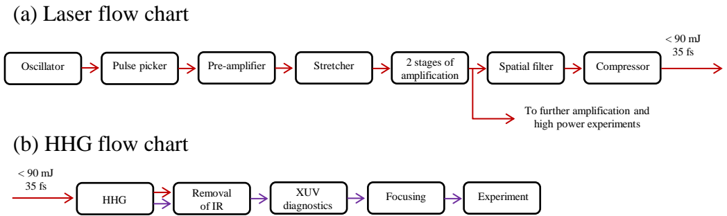
Figure 4.1: Flowchart for: (a) the terawatt Ti:sapphire laser, and (b) the Intense XUV Beamline in Lund. The colours of the arrows indicate whether an IR beam (red) or an XUV beam (violet) propagates between the steps.
