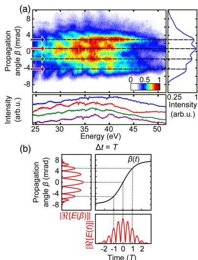
Fig. 2. (a) Measured angularly resolved far-field XUV spectrum in gating conditions ( \Delta t \approx T ). The side panels show the spectrally integrated spatial profile (right) and lineouts (emission angle indicated with arrows in the main panel) of the XUV emission spectra (bottom). (b) Illustration of the time-to-angle mapping of the IR field in gating conditions ( \Delta t = T ) for a CEP of both pulses equal to 0. The bottom panel shows |\Re[E(t)]| , the left panel shows the corresponding |\Re[E(\beta)]| , and the middle one shows the time-to-angle mapping function \beta(t) .
