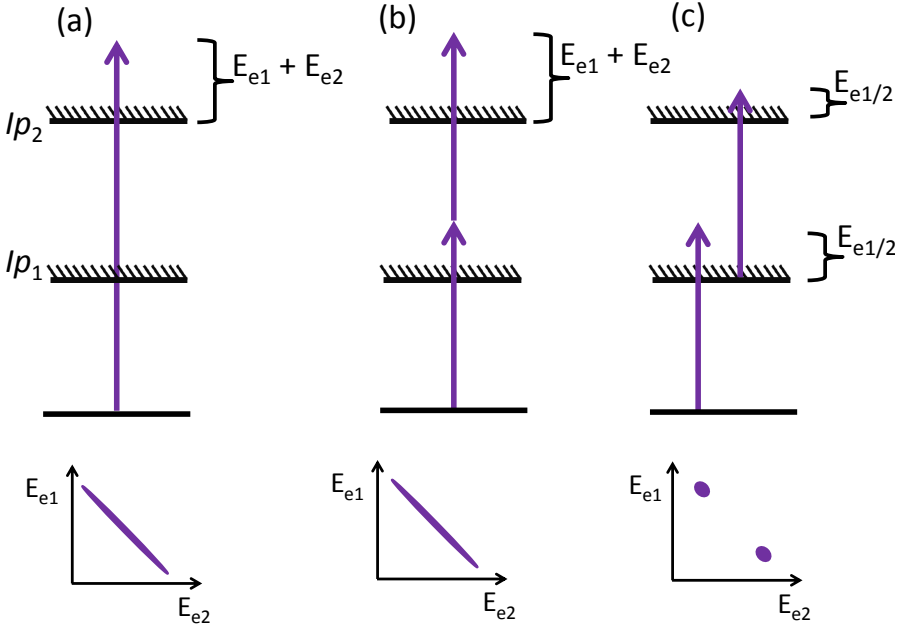
Figure 2.6: Three possible ways to create a doubly charged ion. (a) Absorption of one photon with an energy of E_{\text{ph}} > Ip_1 + Ip_2 . (b) Absorption of two photons that together have energy 2E_{\text{ph}} > Ip_1 + Ip_2 . (c) Absorption of two photons with E_{\text{ph}1} > Ip_1 , E_{\text{ph}2} > Ip_2
