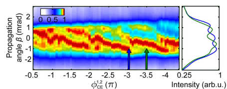
Fig. 4. Spectrally integrated (20–50 eV) spatial XUV far-field profile as a function of CEP (with arbitrary offset) for \Delta t \approx -T . In the right panel, two lineouts with a CEP offset of \pi/2 are shown. The lineout location is marked in the main panel.
