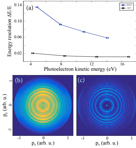
FIG. 6. Experimental results for high resolution electron VMI mode using high-order harmonics to ionize neon. In panel (a) the blue line shows the measured energy resolution for \eta = 0.76 and the black line shows the simulated resolution from Fig. 4. Panels (b) and (c) show the measured detector image and the 3D momentum distribution after inversion.
