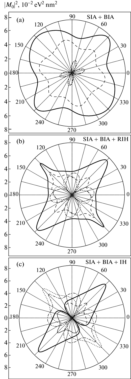
Fig. 2. The absolute value squared of the normalized optical matrix element |M_0|^2 versus the angle \phi for the 1hh-2e transitions with k_\parallel = 0.1 \text{ nm}^{-1} . The solid, dashed, dotted, and dash-dotted curves respectively correspond to the 1hh_b-2e_a , 1hh_a-2e_b , 1hh_a-2e_a , and 1hh_b-2e_b transitions. Light is polarized along the [001] direction.
