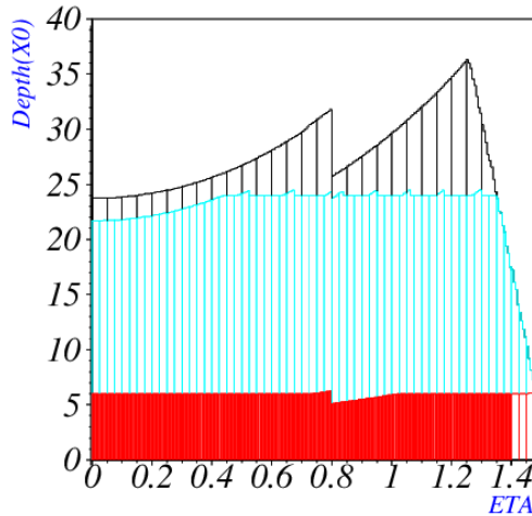
Figure 2.10.: The amount of material traversed by a particle before and in the EM calorimeter, in units of radiation lengths X_0 , as a function of |\eta| . Different colors represent three different longitudinal layers of the EM calorimeter.
