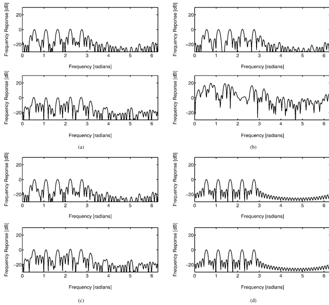
Fig. 1. Frequency responses of the various filters for a set of harmonically related sinusoids in white Gaussian noise at an SNR of -20 dB (top panels) and 20 dB (bottom panels). The designs shown here are (a) SF-APES, (b) SF-Capon, (c) FB-APES, and (d) FB-WNC.
