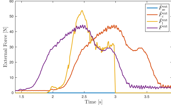
Fig. 10. Predicted external force for a human-guidance situation along the negative z -direction. F^{\text{ext}} denotes the measured external force and \hat{F}_z^{\text{ext}} , \hat{F}_c^{\text{ext}} , and \hat{F}_l^{\text{ext}} denote the zero, constant, and linear predictions of the external force, respectively, for a prediction time of 0.5 s.
