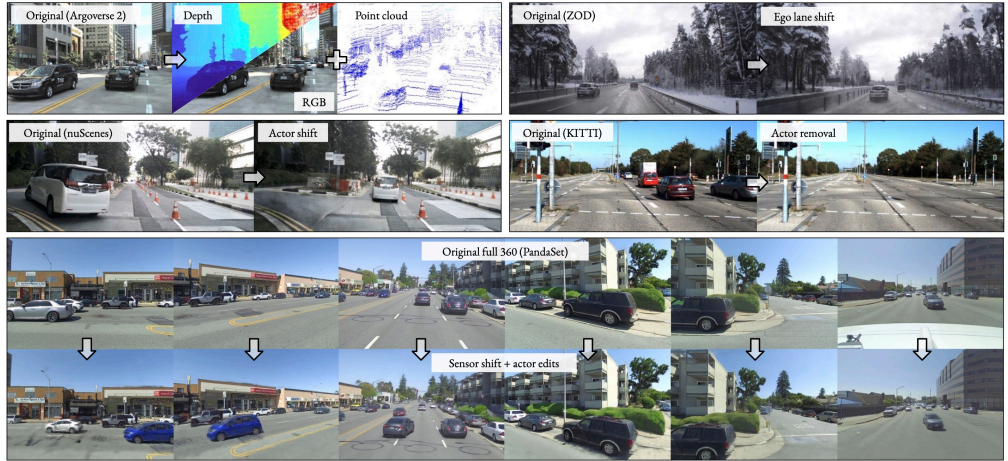
Figure 4.4: Qualitative examples showcasing the capabilities of NeuRAD. At the core is the ability to accurately re-render images, depth maps, and point clouds. By manipulating pose of the view that is rendered one can simulate a novel driving trajectory (shown on ZOD) and/or a different mounting position of the sensor (shown on PandaSet). Furthermore, since NeuRAD uses an explicit decomposition of static scene and dynamic actors, the actors can be removed or modified (shown on KITTI, NuScenes). All capabilities can of course be combined, resulting in realistic surround-consistent novel scenario simulation (shown on PandaSet). Illustration from Paper IV.
