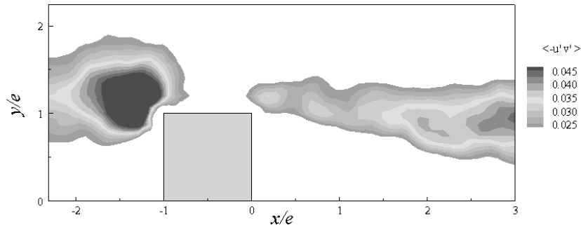
Figure 7: Contours of Reynolds shear stresses, the quantities are normalized by U_0^2 .
