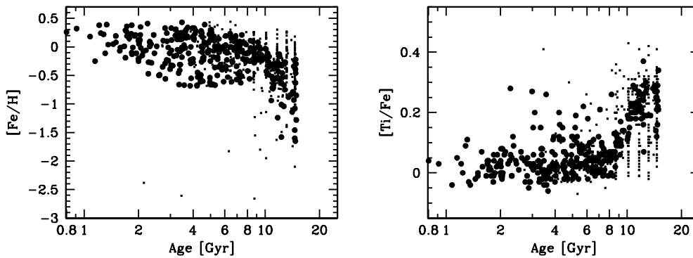
Figure 3. [Fe/H] and [Ti/Fe] versus age. Stars with well-determined ages (difference between upper and lower age estimate less than 3 Gyr) are marked by larger dots.
