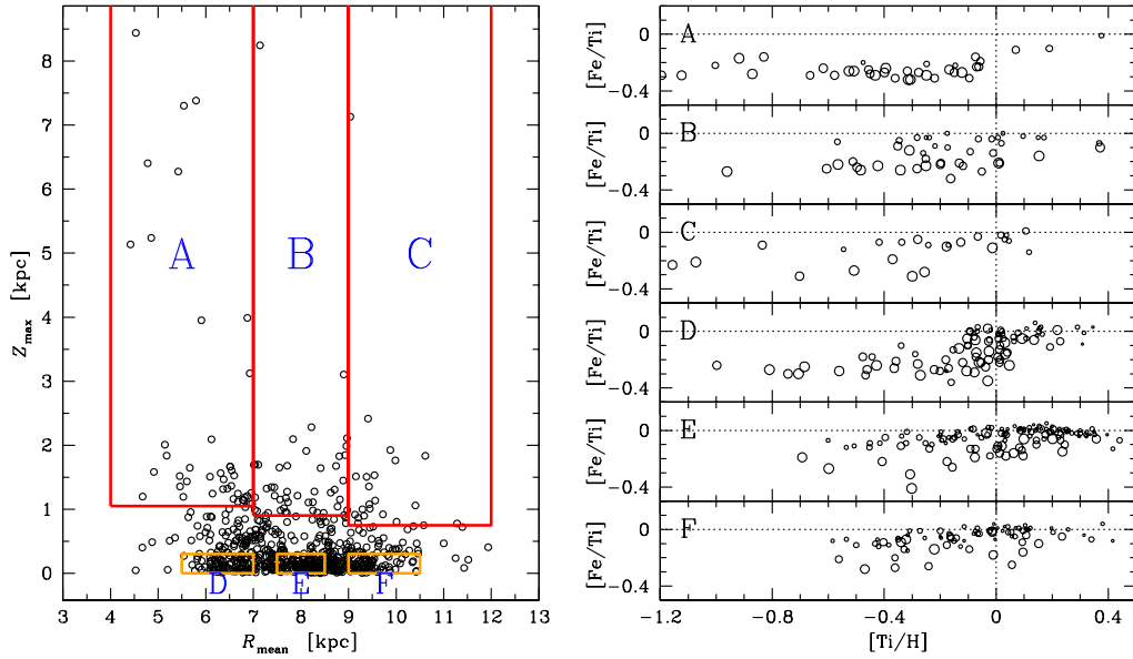
Figure 4. Left: z_{\max} versus R_{\text{mean}} . Right: [\text{Fe}/\text{Ti}]-[\text{Ti}/\text{H}] for stars with orbital parameters as shown in boxes A-F in the plot on the left-hand side. The sizes of the circles have been scaled with the estimated ages of the stars.
