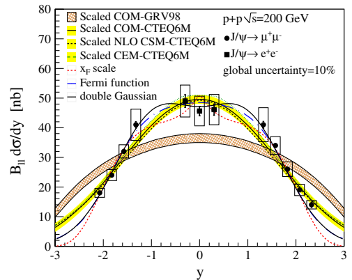
FIG. 21 (color online). Rapidity dependence of the J/\psi yield combining dielectron (solid squares) with dimuon channels (solid circles) along with the fits used to estimate the total cross section. Lines correspond to the three fitting functions described in the text. Also shown are arbitrarily normalized model predictions (NRQCD [51], CEM [52,53], and CSM [17]).
