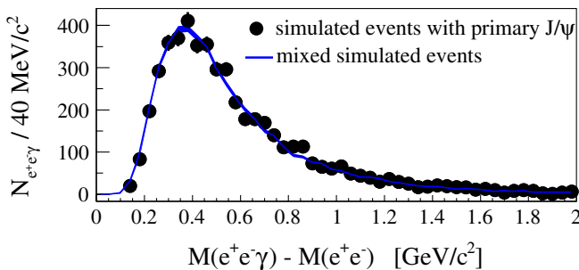
FIG. 14 (color online). Simulated e^+e^-\gamma invariant mass distribution from PYTHIA events containing primary J/\psi decays. The line is the combinatorial background obtained using simulated mixed events from the same sample.
