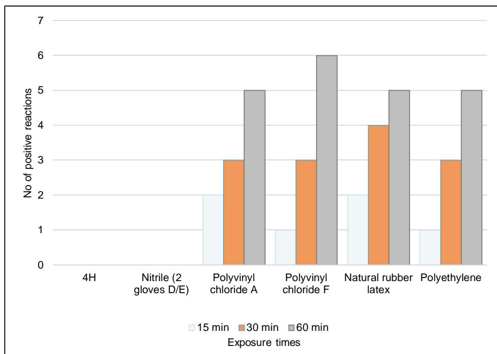
Figure 5. Study I: Number of positive reactions to the glove permeation test with the glove materials tested, related to increasing exposure times.
