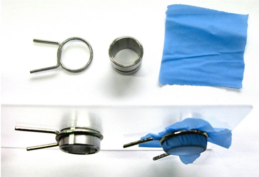
Figure 2 Open chamber test system used in studies I and III.
