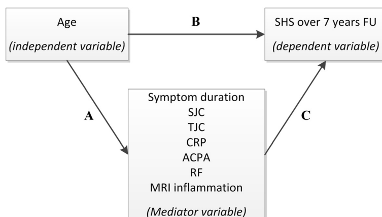
Fig. 1 Schematic overview of the causal paths that were studied using mediation models as described by Baron and Kenny. The figure illustrates two causal paths that lead to an outcome. A direct path from independent variable ( b ) and an indirect path from an independent to a dependent variable through a mediator variable ( a,c ). To test mediation three tests have to be performed according to Baron and Kenny [36]. 1) The mediator variables were regressed on the independent variable ( a ), the independent variable should significantly affect the mediator variables. 2) regression analysis of the dependent variable on the independent variable was done ( b ); in this analysis the independent variable must significantly affect the dependent variable. 3) The dependent variable was regressed on the independent and mediator variable ( b and c ). When mediation occurs the mediator variable significantly affects the dependent variable and the effect of the independent variable on the dependent variable is closer to zero. In this study we tested whether different mediators could influence the effect of age on radiographic joint damage. The tested mediators were symptom duration at diagnosis, swollen joint count ( SJC ), tender joint count ( TJC ), C-reactive protein ( CRP ), anti-citrullinated protein antibody ( ACPA ), rheumatoid factor ( RF ), and inflammation detected on magnetic resonance imaging ( MRI ). SHS Sharp-van der Heijde score
