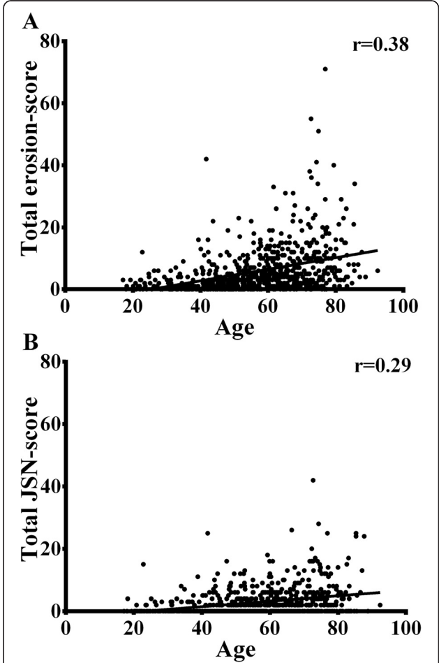
Fig. 3 Correlation between age and Sharp-van der Heijde erosion (a) and joint space narrowing scores (JSN) (b) at baseline
