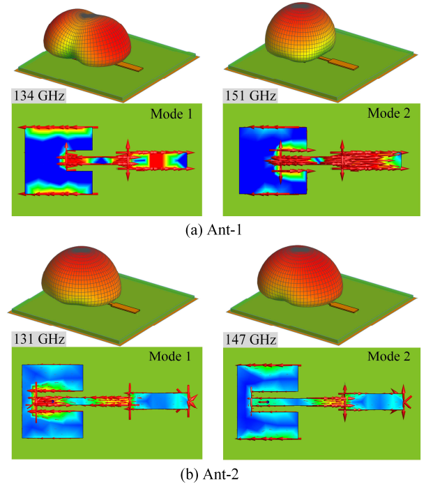
Fig. 4. Modal far-field radiation patterns and current distributions for (a) Ant-1 and (b) Ant-2.
