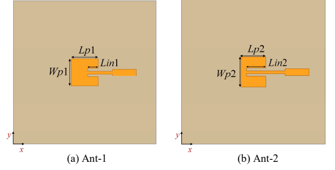
Fig. 2. Top view of the two antenna structures on a single board. ( Lp1 = 0.57 , Wp1 = 0.57 , Lin1 = 0.22 , Lp2 = 0.51 , Wp2 = 0.66 , Lin2 = 0.4 . Unit: mm)
