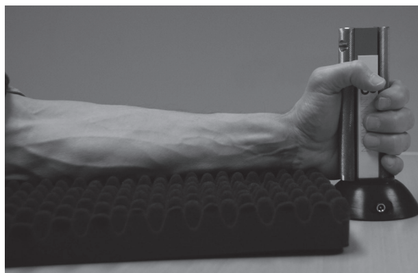
Fig. 2. Set-up and testing position for isometric grip strength using the Grippit dynamometer.
