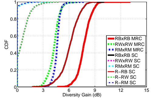
Fig. 6. Rural convoy: Both TX/RX vehicles are well aligned so the RW \times RW and RM \times RM links provide diversity gain also with SC. However, the RB \times RB combination has the best performance since it provides 6 dB and 8 dB gain for SC and MRC, respectively, for more than 50% of the time.
