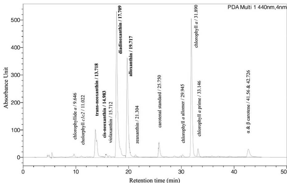
FIG. 1. HPLC chromatogram of Gonyostomum semen with identified pigment peaks and retention times. Pigments, written in bold, have not been found in marine raphidophytes.
