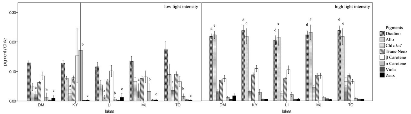
FIG. 6. Means of accessory pigments per chlorophyll a in two pooled light treatments: low light intensity (5, 10, and 25 \mu\text{mol photons} \cdot \text{m}^{-2} \cdot \text{s}^{-1} ) and high light intensity (150 and 200 \mu\text{mol photons} \cdot \text{m}^{-2} \cdot \text{s}^{-1} ). Strains are grouped by lake of origin: LI, Liasjön; DM, Dammen; MJ, Mjotrasket; TO, Torsjön; KY, Kylänalainen. Means with identical letters are not significantly different. Error bars represent SE.
