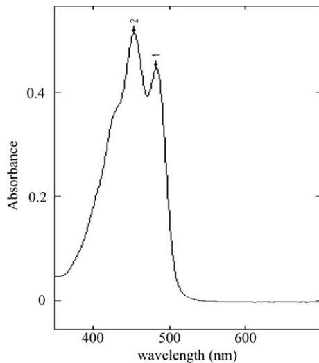
FIG. 4. UV-Vis spectrum of alloxanthin in acetone of Gonyostomum semen , 2 = 454 nm, 1 = 484 nm.
