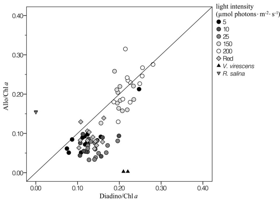
FIG. 5. Correlation between alloxanthin/Chl a and diadinoxanthin/Chl a in Gonyostomum semen (several light conditions), Vacuolaria virescens and Rhodomonas salina . Black line corresponds to equal distribution of both pigments in relation to chl a .
