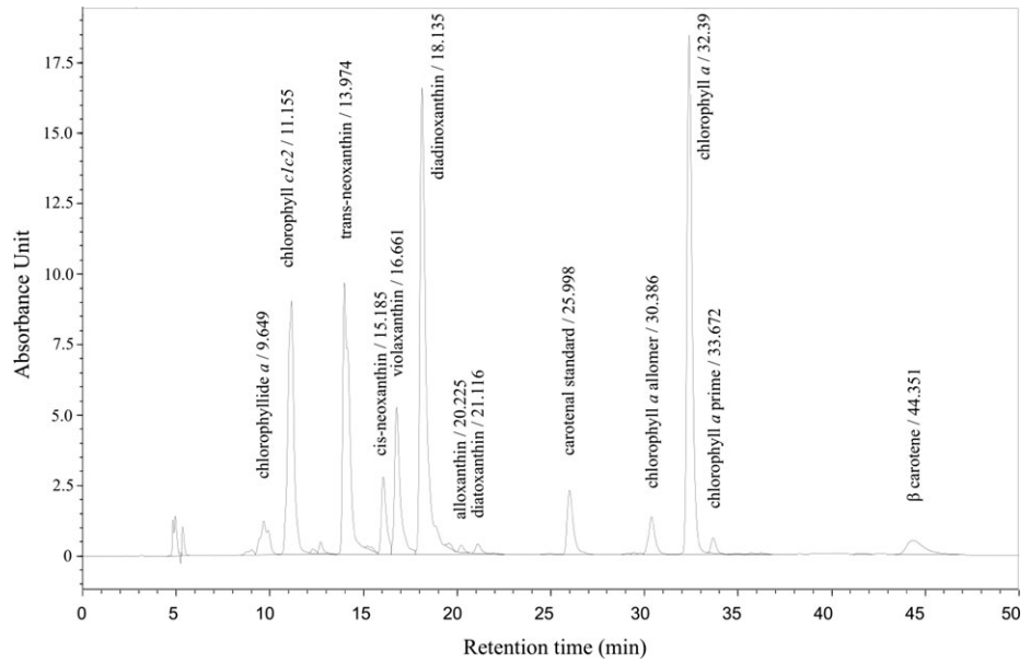
FIG. 2. HPLC chromatogram of Vacuolaria virescens with identified pigment peaks and retention times.
