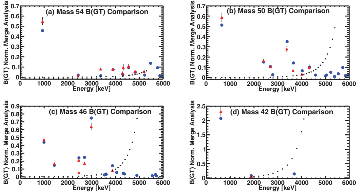
FIG. 18. (Color online) Comparison of B(\text{GT}) values obtained in the present analysis (solid red triangles) and those from the ( ^3\text{He}, t ), CE reactions (solid blue circles) as a function of excitation energy in the daughter nucleus. To derive the absolute B(\text{GT}) values from the CE reaction data, the “merged analysis” was used (see text). The dots show the sensitivity limit in the present experiment; for masses 54 and 50 the limit stops at the energy where proton decay is expected to dominate (see text).
