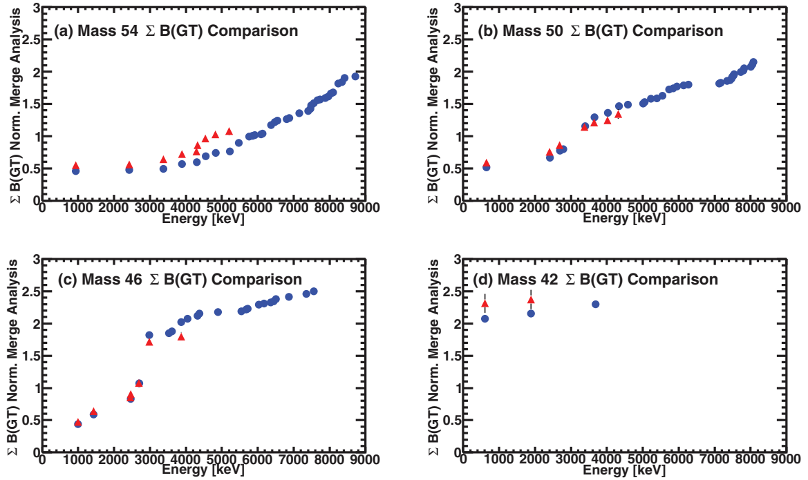
FIG. 19. (Color online) Comparison of accumulated B(GT) values obtained in the present analysis (solid red triangles) and those from the (^3\text{He}, t) , CE reactions (solid blue circles) as a function of excitation energy in the daughter nucleus. To derive the absolute accumulated B(GT) values from the data of CE reactions, the “merged analysis” was used (see text).
