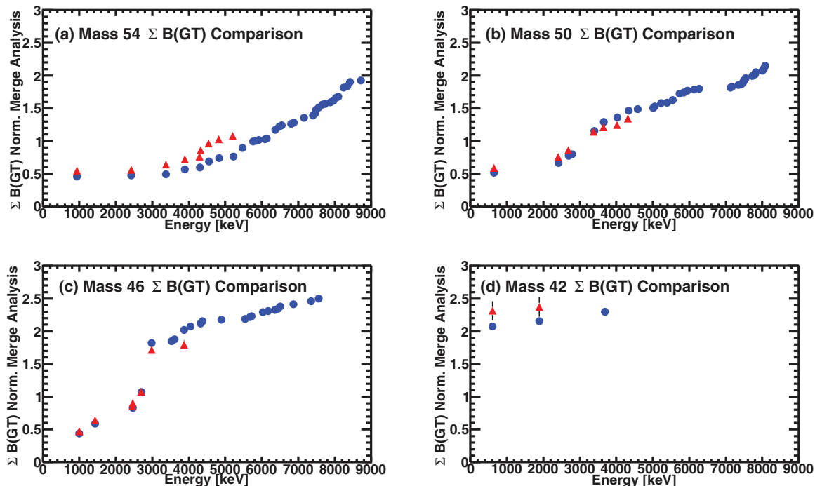
FIG. 19. (Color online) Comparison of accumulated B(GT) values obtained in the present analysis (solid red triangles) and those from the ({}^3\text{He},t) , CE reactions (solid blue circles) as a function of excitation energy in the daughter nucleus. To derive the absolute accumulated B(GT) values from the data of CE reactions, the “merged analysis” was used (see text).
