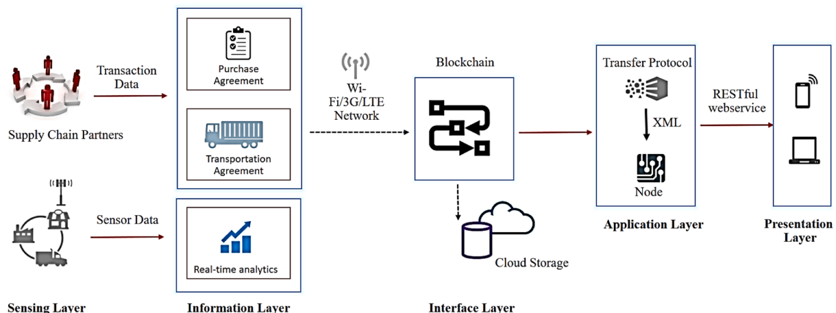
Fig. 7. Schematic of proposed blockchain system architecture.
