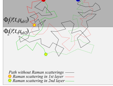
Figure 1. Two-layer reflectance geometry with exemplary photon paths and Raman scattering events.
