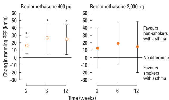
Fig. 2. Mean (95%) difference between non-smokers and smokers with asthma in change in morning PEF (L/min) on different doses of inhaled beclomethasone. * P<0.01 for smokers with asthma vs non-smokers with asthma. 26 Reproduced from Thorax, Tomlinson JEM, McMahon AD, Chaudhuri R, Thompson JM, Wood SF, Thomson NC. Efficacy of low and high dose inhaled corticosteroid in smokers versus non-smokers with mild asthma. 60:282-287. 2005. With permission from BMJ Publishing Group Ltd.
