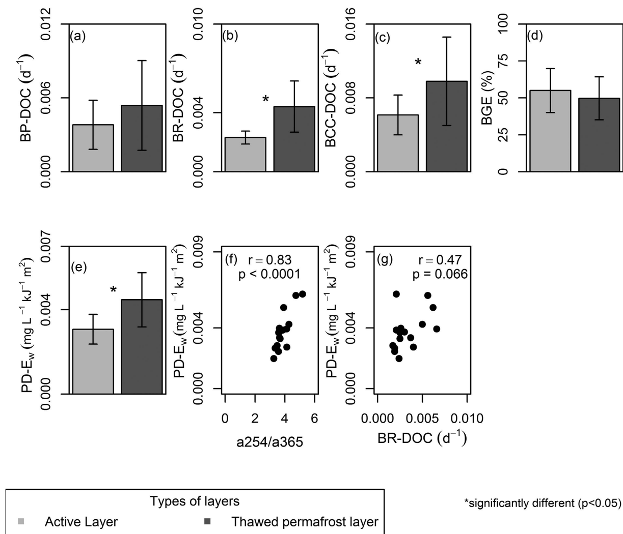
Figure 2. DOC degradation in the active layer ( n = 8 ) and the thawed permafrost layer ( n = 8 ). For bio-degradation, the plots show (a) Bacterial production normalized to DOC (BP-DOC), (b) Bacterial respiration normalized to DOC (BR-DOC), (c) Bacterial carbon consumption normalized to DOC (BCC-DOC), and (d) Bacterial growth efficiency (BGE). In the plot (e) the DOC degradation rate per unit irradiation absorbed (PD-E w ) is shown. Error bars indicate standard deviation of the mean. The plot (f) absorption ratio (a254/a365) vs PD-E w ( n = 16 ) and (g) BR-DOC vs PD-E w ( n = 16 ) are Pearson correlation. See sections 2.3 and 2.4 for details of bio- and photo-degradation experiments, respectively.
