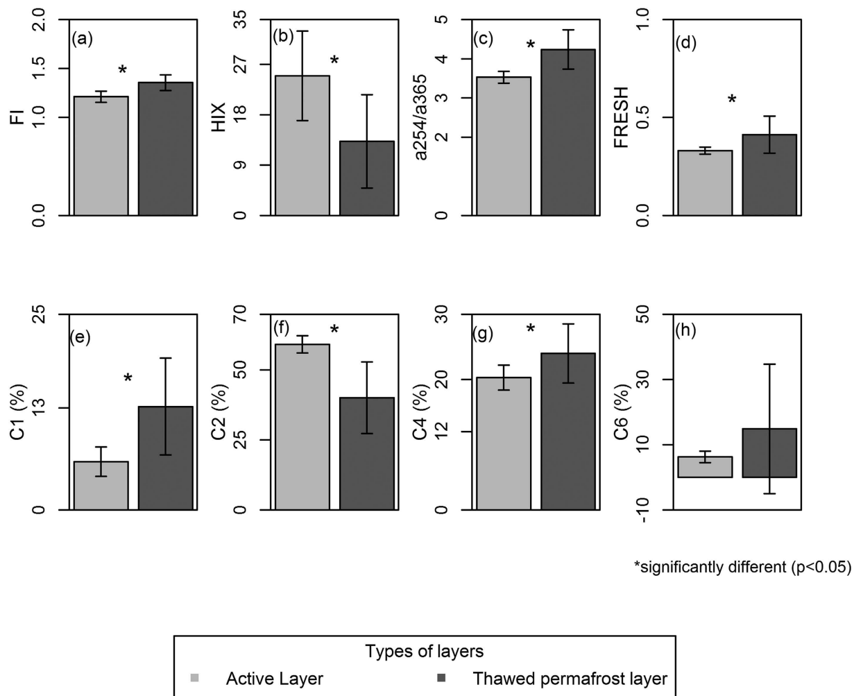
Figure 1. Dissolved organic carbon (DOC) composition in the active layer (n = 8) and the thawed permafrost layer (n = 8). The plots show (a) Fluorescence index (FI), (b) Humification index (HIX), (c) absorbance ratio (a254/a365), (d) Freshness index (FRESH), (e) Humic-like fluorescence component (C1), (f) Humic-like fluorescence component (C2), (g) Humic-like fluorescence component (C4), and (h) protein-like fluorescent component (C6) are the DOC composition. Error bars indicate standard deviation of the mean. See section 2.1 for details of core collection and incubation.
