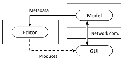
Figure 4.4: Architecture for inverted development approach. Through strict separation of concerns, the GUI and model are run independently on separate devices. Since the model is always-on, the editor can read it in real-time during the design process.
