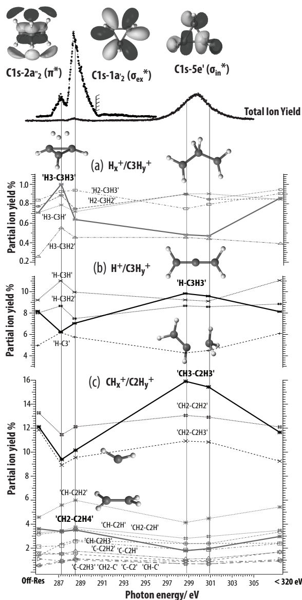
Figure 5.10: Partial ion yield of dissociation channels following cyclopropane C1s-2a''( \pi^* ), C1s-1a 2 '( \sigma_{ex}^* ), and C1s-5e'( \sigma_{in}^* ) resonances.
