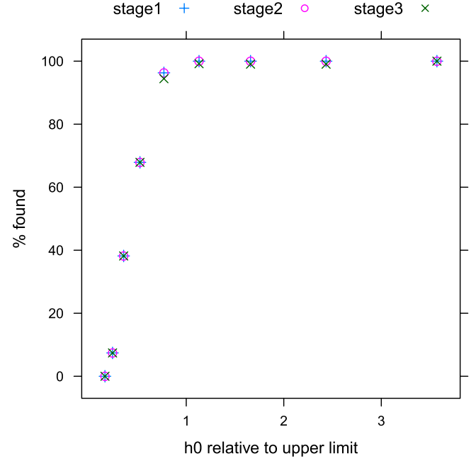
FIG. 8 (color online). Injection recovery from semicoherent analysis stage (crosses), after the first loosely coherent follow-up (circles) and after the second stage of loosely coherent follow-up (diagonal crosses). The injected strain divided by the upper limit in this band (before injection) is shown on the x axis. The percentage of surviving injections is shown on the y axis.
