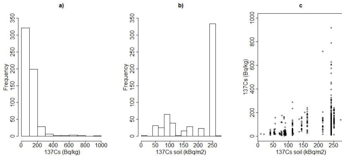
Fig 1. Exposure distributions of a) ^{137}\text{Cs} Whole body concentration (WBC, Bq/kg), b) ^{137}\text{Cs} in Soil(kBq/m 2 ), and c) the correlation between ^{137}\text{Cs} in soil (x-axis) and ^{137}\text{Cs} WBC (y-axis). (n=566).
