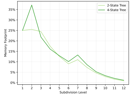
Figure 5: Average footprint reduction over all scenes and subdivision levels.
