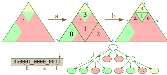
Figure 3: Overview of the look-up algorithm from the micromap tree representation.
