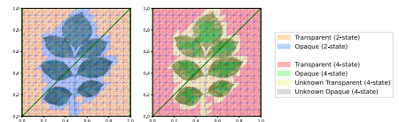
Figure 5: Two examples of a micromapped primitive using the 2-state (left) and 4-state (right) modes.
