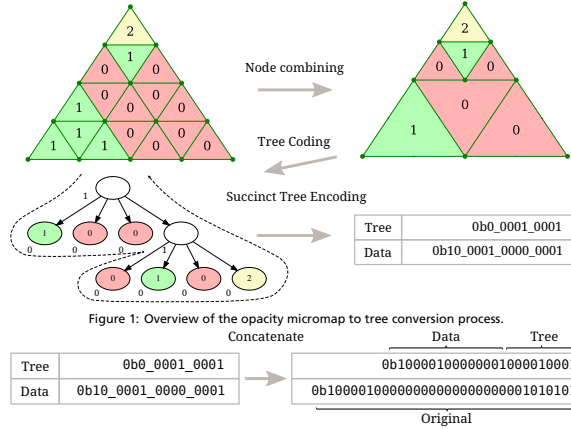
Figure 2: Bitwise comparison of the original opacity micromap and the tree from the above example.
