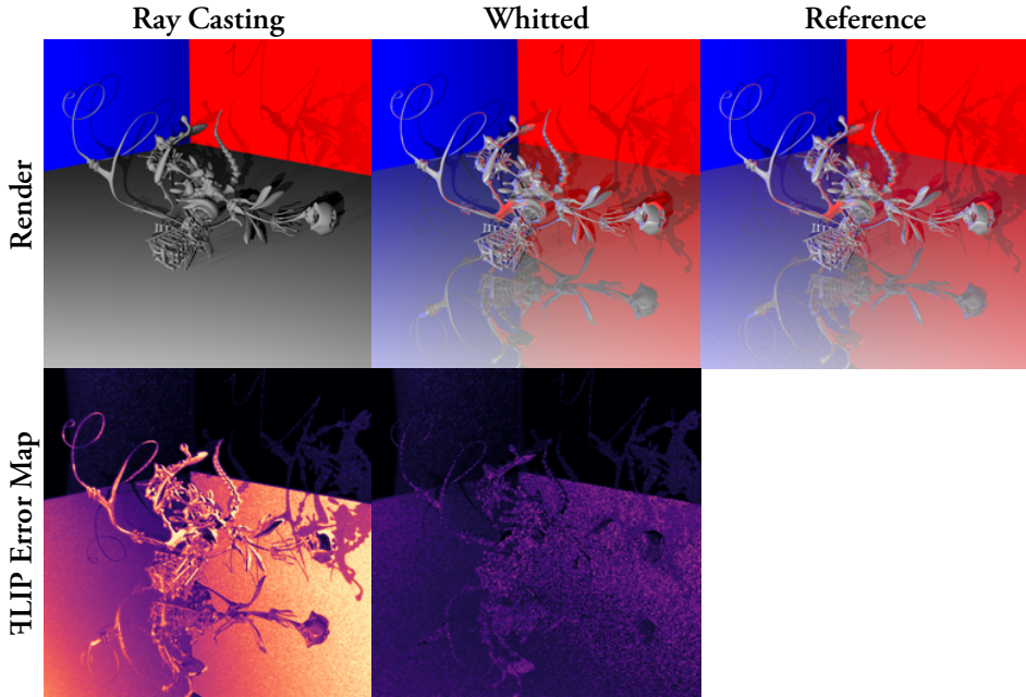
Figure 39: The \mathcal{FLIP} [2] metric applied to the ray casting and Whitted approximations to the rendering equation from figure 16.
