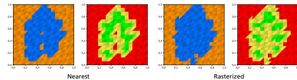
Figure 3: The micromap quality is a user parameter: A simple micromap may use the alpha nearest subtriangle vertex, but to avoid missing small features, each microtriangle should be rasterized. Notice the missing stem in two leftmost images!
