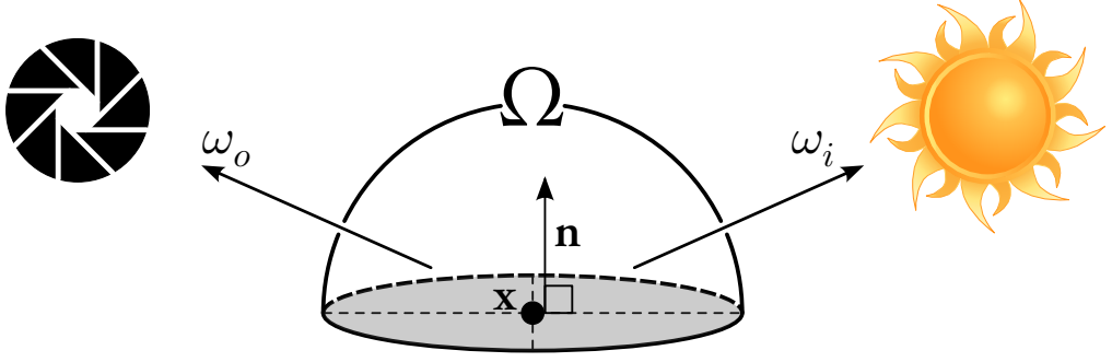
Figure 15: A schematic overview of the so-called Rendering Equation. The Light that leaves a point \mathbf{x} with surface normal \mathbf{n} depends on the light from all possible directions \omega_i on the hemispherical domain \Omega , modulated by the material itself at this point.
