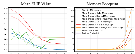
Figure 3: Mean FLIP error and memory footprint (MB) at increasing subdivision levels.
