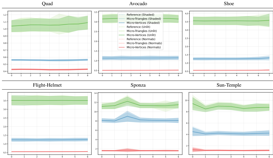
Figure 8: Frame runtime results in milliseconds (ms).
