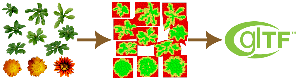
Figure 44: The extensibility of the glTF format makes it relatively easy to add new things to it, such as opacity micromaps : An object that similar to alpha-masking can selectively mask out objects, but at a much lower cost, something that is explored more thoroughly in Paper III. In this example, opacity micromaps (center) are derived from alpha textures from the Sponza [92] scene (left) and then stored in a glTF file, here symbolized with its logo (right). The rendered results from this process can be seen in figure 45.
