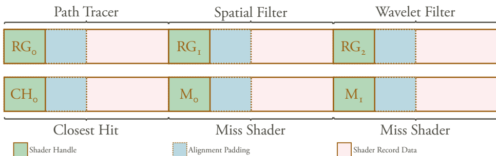
Figure 34: Visualization of the shader binding table (SBT) modified to perform non-ray-tracing related work, such as spatio-temporal filtering. Instead of switching between several different computer shader pipelines, a single ray-tracing pipeline can switch between the different shaders that are used to implement image filtering algorithms, such as a spatial and wavelet filter in this case.
