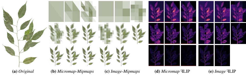
Figure 5: Mipmaps created for a micro-triangle based color micromap by averaging the color of the 4 underlying child nodes (b), the equivalent image-based mipmaps (c) as well as the TLIP error maps between each mipmap level and the original texture (d and e). Note that two triangles are used to create a comparable rectangle which consequently have two colors at the highest mip-level. Thus, to make the visual comparison fairer to image based mipmaps, we drop the highest mip-level and shift the hierarchy accordingly.
