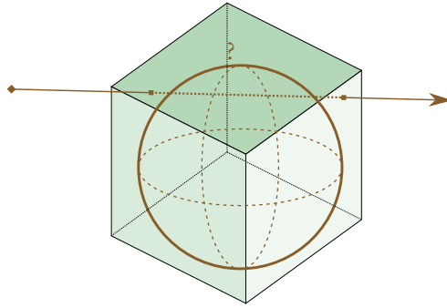
Figure 32: The acceleration structure for the ray-tracing pipeline only store the Axis-Aligned Bounding Boxes (AABBs) around user defined objects. The Intersection shader is used to determine if a ray that intersects such a box also intersects with the contained object, such as the sphere shown in this case.
