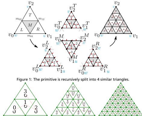
Figure 2: The first three subdivision levels.
