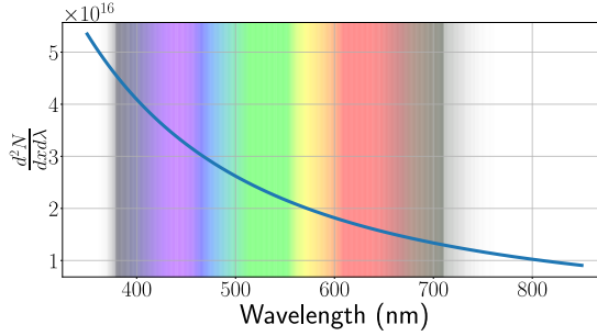
Figure 3: Example of how equation 2 maps particle energy to photons. Depicted here for an electron moving through heavy water ( n \approx 1.328 ) at a speed of 0.8c_0 , assuming that \mu(\lambda) = 1 .
