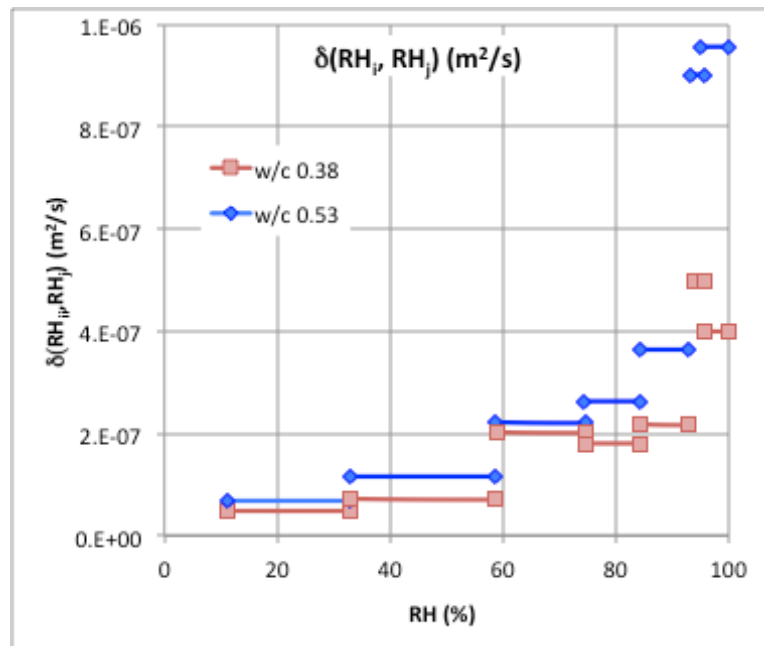
Fig. 33 The average moisture transport coefficient \delta_j(RH_i, RH_j) in small RH intervals for the two mortars.
