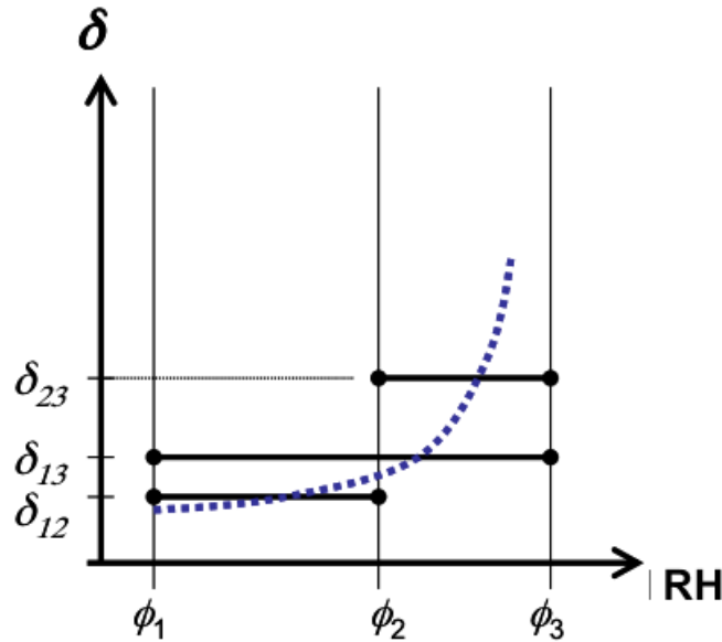
Fig. 32 The moisture transport coefficient \delta(\text{RH}) (dashed curve) and the average \delta_j(\text{RH}_i, \text{RH}_j) in different intervals
