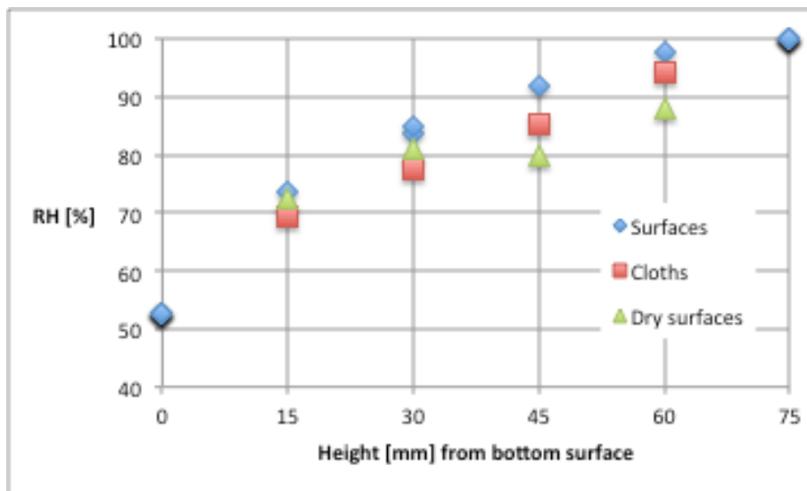
Fig. 36 Measured steady-state RH between the five discs
