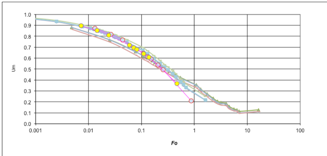
Fig. 52 The weight loss curves for 15 mm and 45 mm mortar I discs drying two ways, compared to the curves for the rolls (circles) with 2L=75 mm.
