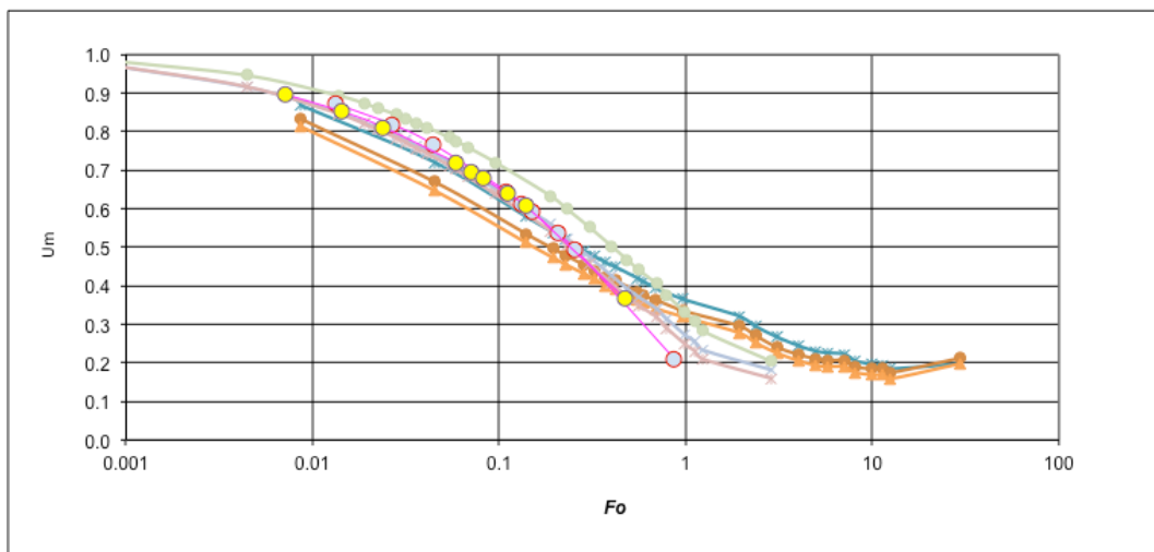
Fig. 53 The weight loss curves for 15 mm and 45 mm mortar II discs drying two ways, compared to the curves for the rolls (circles) with 2L=75 mm.
