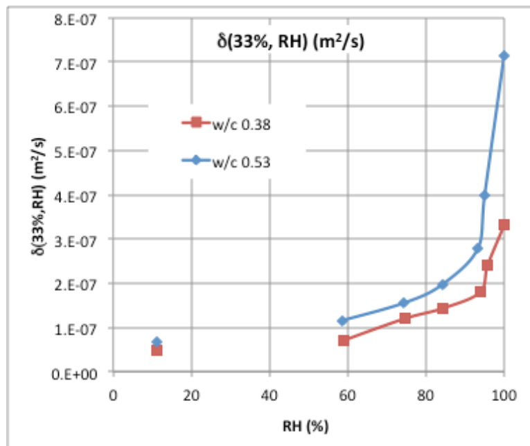
Fig. 31 The average moisture transport coefficient \delta(33, \Phi_2) as a function of the RH-interval with 33 % RH on one side and \text{RH} = \Phi_2 on the other side.
