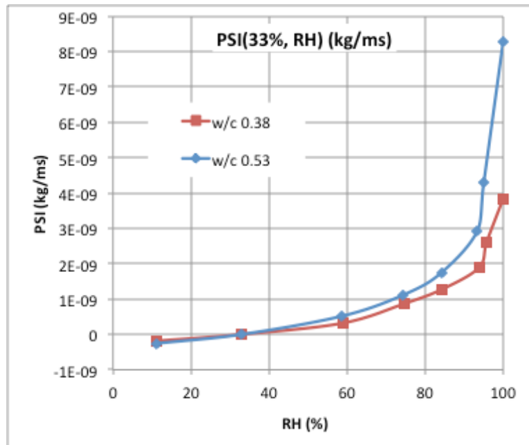
Fig. 30 The fundamental potential PSI as a function of the RH-interval with 33 % RH on one side and RH on the other side.
