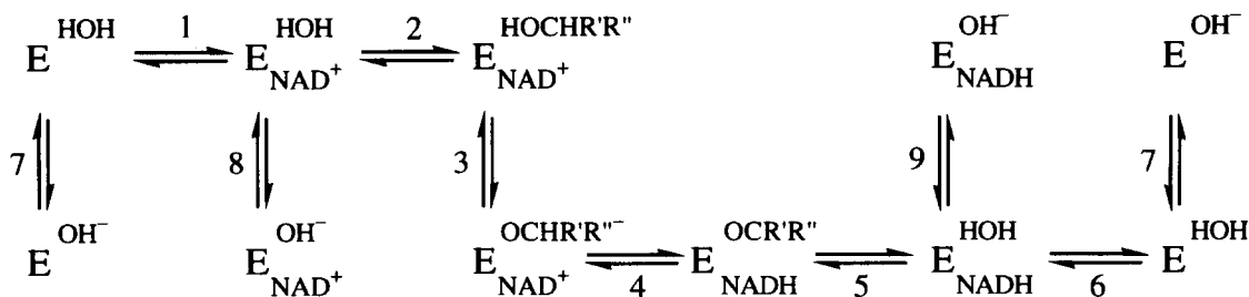
Fig. 1. Reaction mechanism proposed by Pettersson (1987). E denotes the enzyme.
