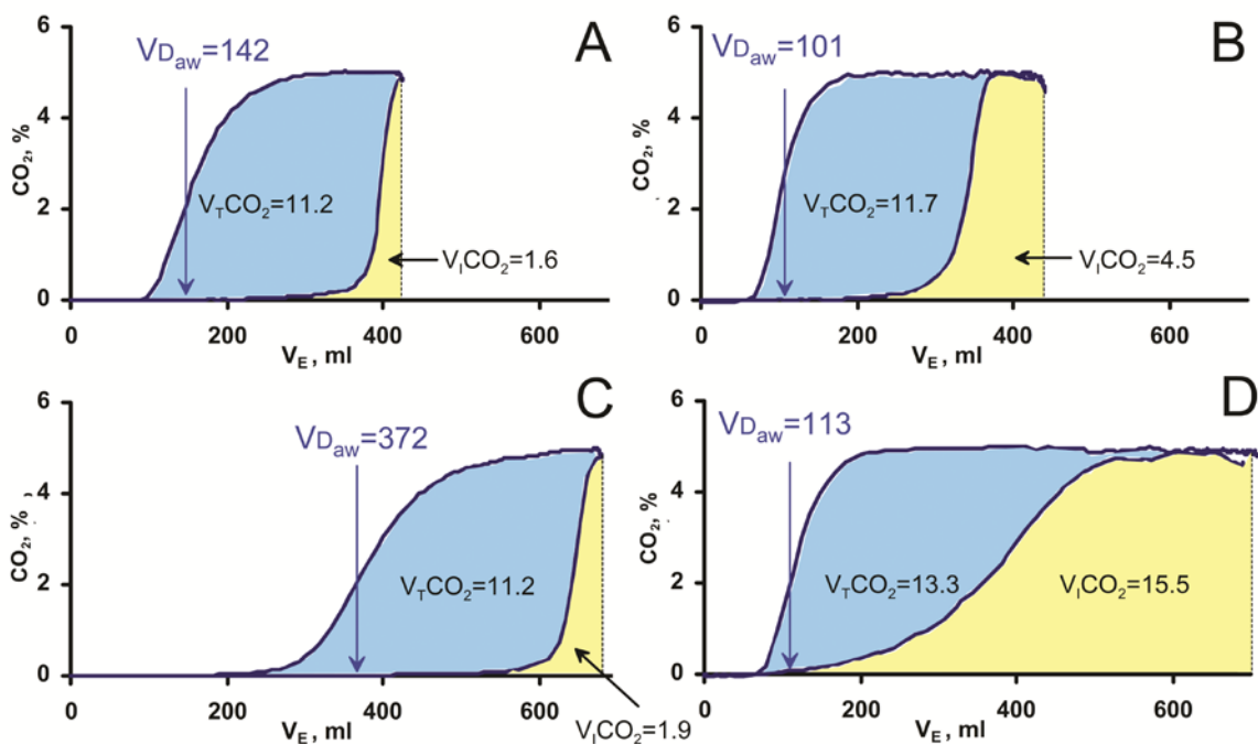
Fig 4 Single breath tests for \text{CO}_2 (SBT- \text{CO}_2 ) with an HME (A and B) or active ACD (C and D) registered on ventilator (A and C) or lung (B and D) side of the device, respectively. All volumes in millilitres. The volume of \text{CO}_2 eliminated during the breath ( V_T\text{CO}_2 , blue area) and inspired ( V_I\text{CO}_2 , yellow area) is indicated. Apparent airway dead space ( V_{D_{aw}} ) is indicated by the vertical arrow. SBT- \text{CO}_2 was studied after adjustment of tidal volume to maintain isocapnia and in steady state with respect to \text{CO}_2 elimination. As illustrated in panel C, the effect of the ACD is analogous to a large increase in V_{D_{aw}} observed on the ventilator side of the device. In panel D this is reflected by the yellow area, representing a large volume of re-inspired \text{CO}_2 from the ACD.
