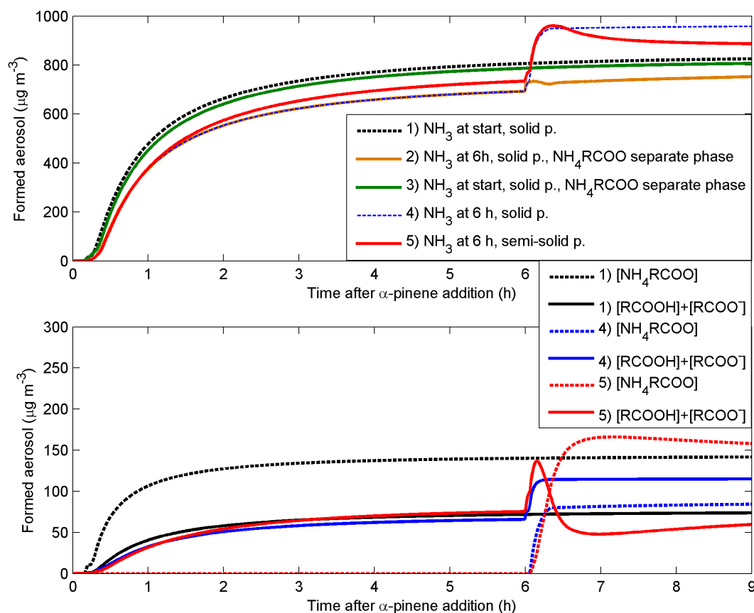
Figure 10. Modelled SOA mass formation for \alpha -pinene– O_3 – NH_3 – CO experiments with 200 ppb NH_3 added at the start or after 6 h of aging. For all simulations, SIMPOL was used to estimate the vapour pressures of the organic compounds. The SOA particles were either treated as completely solid (no mixing between particle layers) (simulation 1–4) or semi-solid with D_{0,monomer,SOA} = 10^{-15} \text{ cm}^2 \text{ s}^{-1} , D_{0,ammonium} = 10^{-13} \text{ cm}^2 \text{ s}^{-1} and D_{0,NH_4RCOO} = 0 \text{ cm}^2 \text{ s}^{-1} (simulation 5). For simulations 2 and 3 we assume that the NH_4RCOO salts form a separate phase which other organic compounds cannot dissolve into.
