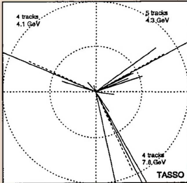
Figure from the TASSO experiment at DESY in Hamburg, which demonstrated the existence of gluons, thereby confirming the theory of QCD. The figure shows three particle showers from a quark, an antiquark and a gluon created by the collision between an electron and a positron.
