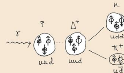
Schematic illustration of the spin flip of a quark in a nucleon.
