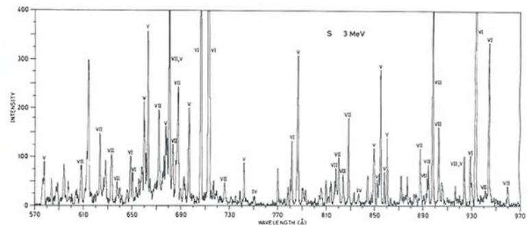
Spectral lines from a beam of positively charged sulphur ions: S^{3+} , S^{4+} , S^{5+} , S^{6+} .
