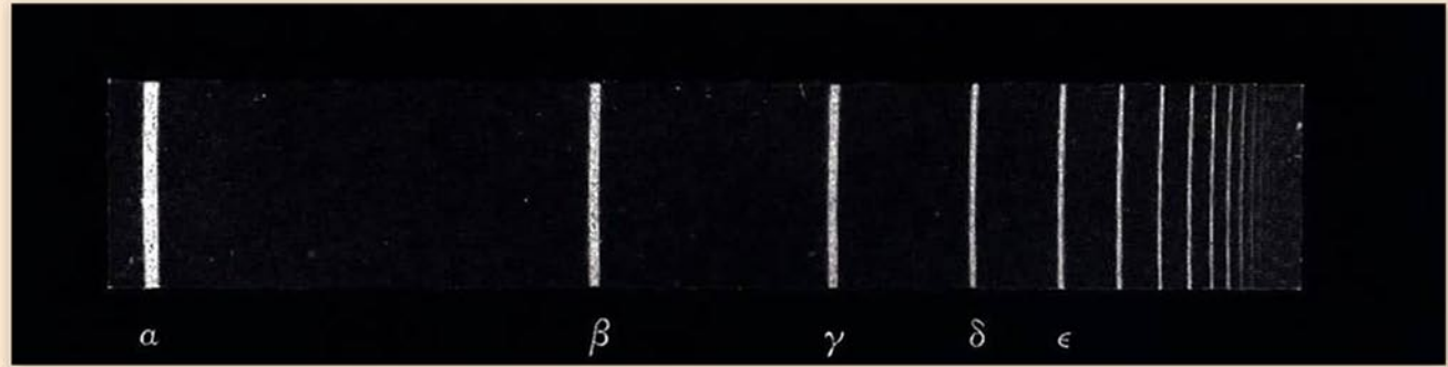
The simplest series of spectral lines had been observed in hydrogen.
