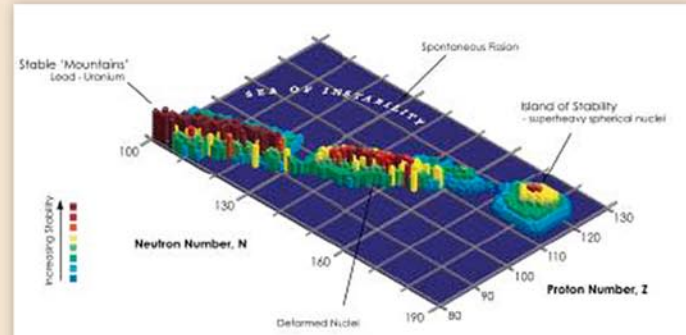
A three-dimensional image showing the theoretical peninsula of more stable nuclei around Z=114-126 and N=178-184 (from 2011).
