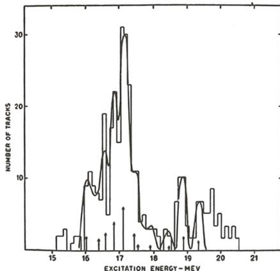
Spectrum showing the energy distribution of photoprotons from an oxygen molecule.
