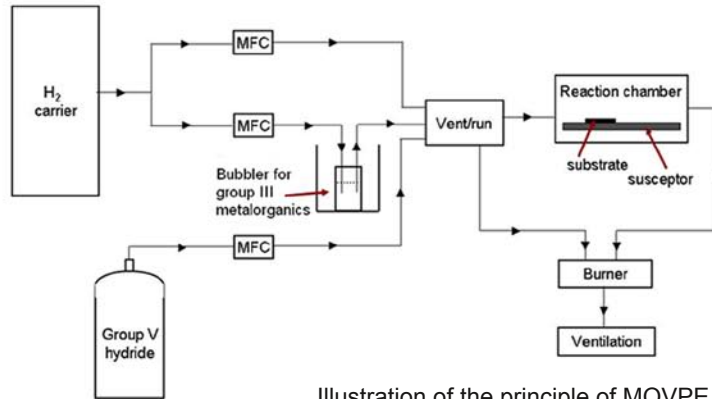
Illustration of the principle of MOVPE.
