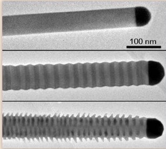
Nanowires with and without a heterogeneous structure.
