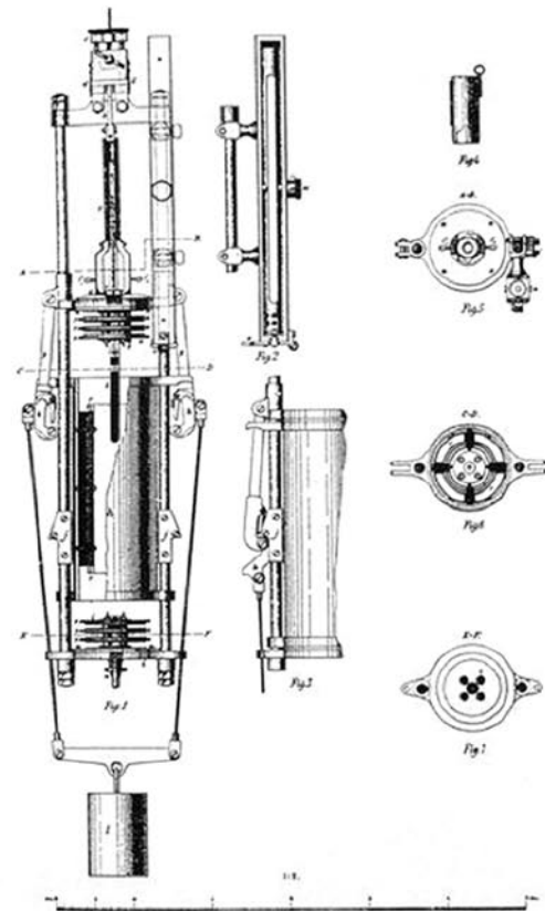
Ekman's design for an ocean current meter.
