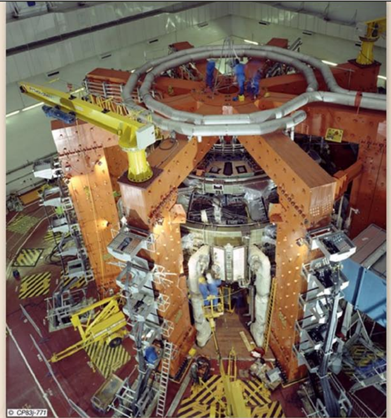
The JET tokamak at Culham, UK.
