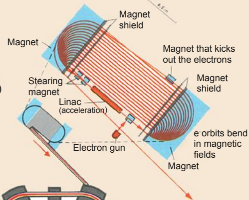
100 MeV Microtron (acceleration of electrons)
