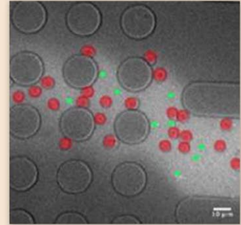
An example of a lab on a chip used here to sort particles. The figure shows a so-called bumper array , which sorts particles according to size and shape based on the path they take through the device.
