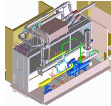
The high-pressure combustion test rig.
