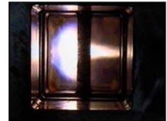
Photograph of a pilot flame in one of the burners tested in the high-pressure combustion rig.
