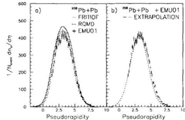
Experimental data and simulated results of Pb-Pb collisions.
