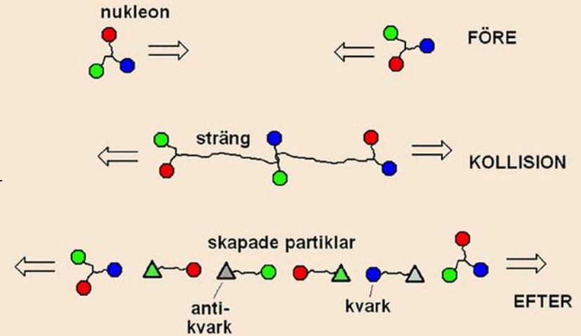
Schematic illustration of the fragmentation of gluon strings according to the Lund Model.
