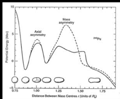
A diagram and ceramic model, by Lisa Larsson, showing the variation in the potential energy of the atom in the process leading to fission, illustrating that fission is easier if the two fragments have different masses.
