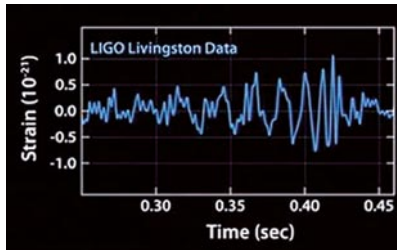
The detection of a gravitational wave.
