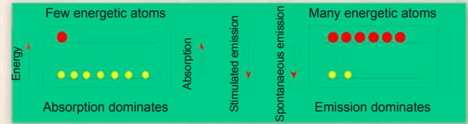
Various atomic systems. Normal population. Inverted population.
