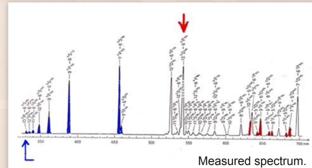
Laser spectroscopy in Cs I.
