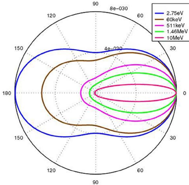
The Klein-Nishina distribution of photon scattering angle at different energies.
