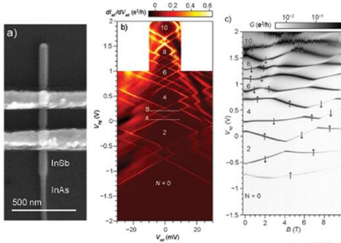
Spintronics
