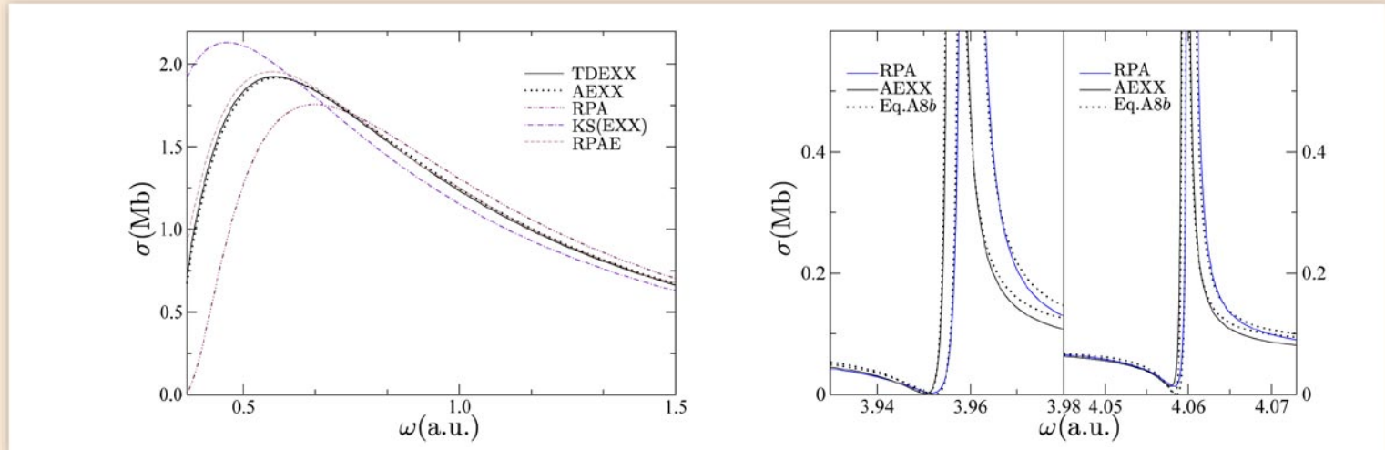
Top left: Photoionization cross section for Be after the first ionization threshold.
