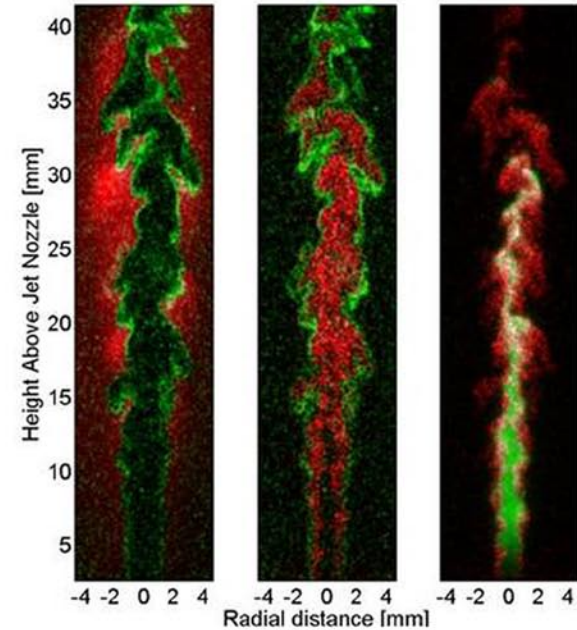
This figure shows LIF measurements of OH (warm product), CH (flame edge), CH 2 O (cool zone) and traces of uncombusted fuel (cold zone) in a turbulent jet flame. Each image contains two products. Left: OH (red) and CH (green), Middle: CH 2 O (red) and CH (green), Right: CH 2 O (red) and fuel (green).
