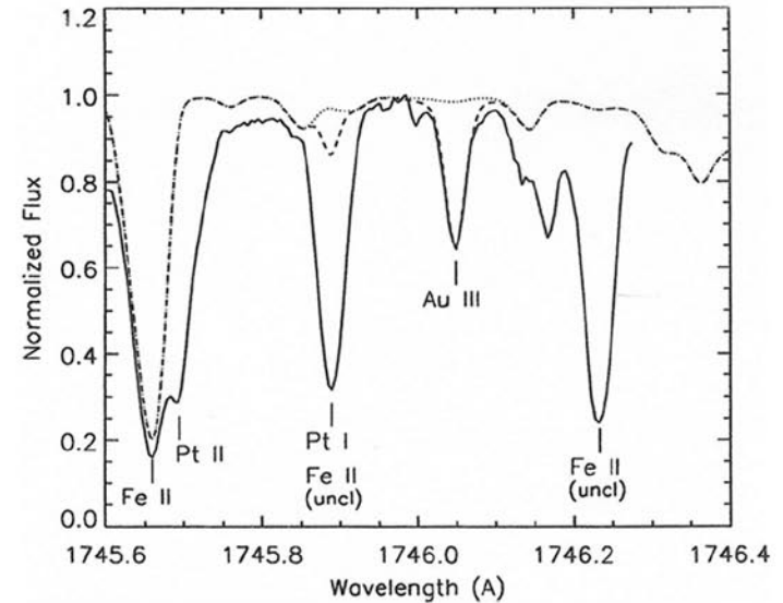
Details in the UV spectrum from Chi Lupi showing spectra lines from Au, Pt, and Fe.
