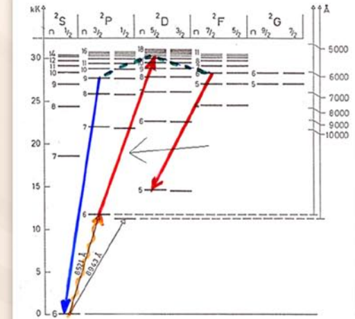
Laser spectroscopy in Cs I.
