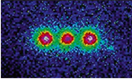
Three Be ions.
