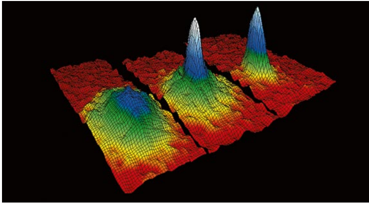
Formation of a Bose-Einstein condensate.
