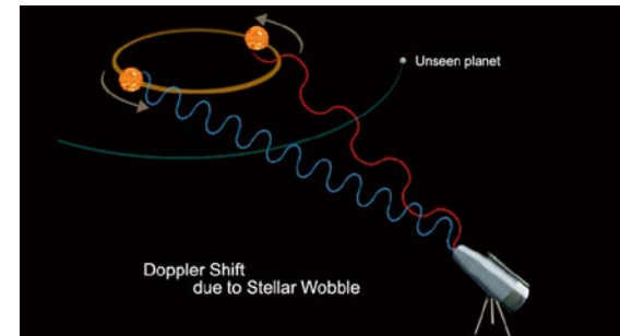
Observation of planets using the Doppler technique.
