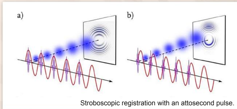
Electrons leaving the nucleus of the atom.
