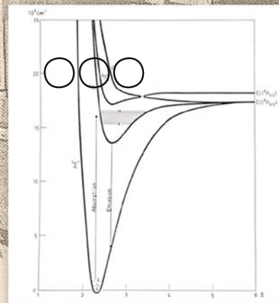
Absorption and emission of an iodine chloride molecule.
