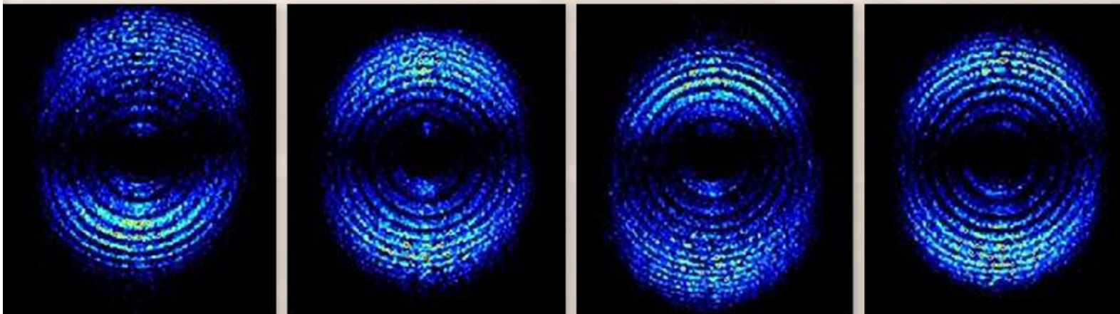
Electrons leaving the nucleus of the atom.
