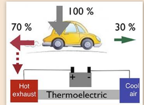
Thermoelectricity
