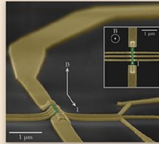
The Hall effect in a single nanowire.
