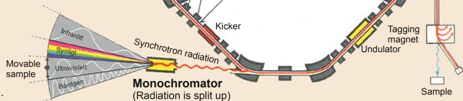
Sketch of the MAX I ring.
