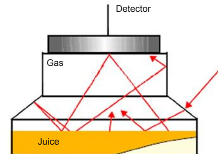
Measurements of gas inside a package of juice.
