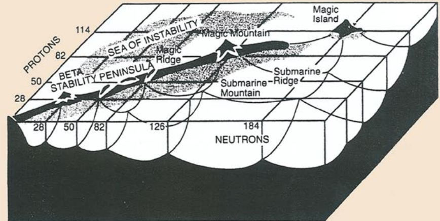
A peninsula of stable nuclei and the predicted island of superheavy nuclei.
