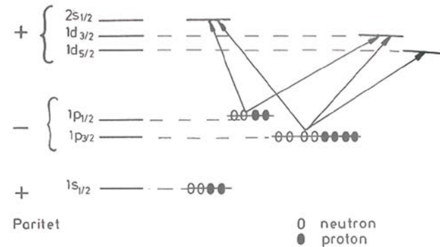
A particle-hole transition according to the shell model.
