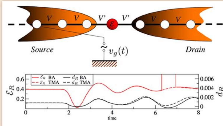
Double occupation in a nanoscopic scale conductor, according to the work of Puig von Friesen, Verdozzi, and Almladh in 2011.
