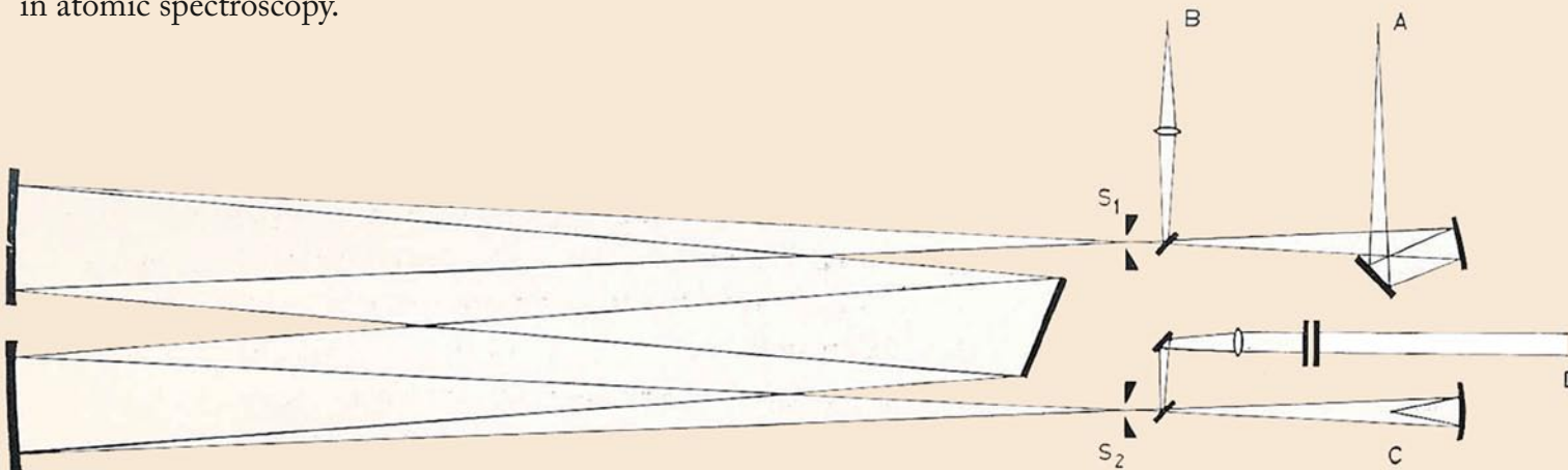
A spectrometer for infrared radiation, constructed in Lund in 1969.
