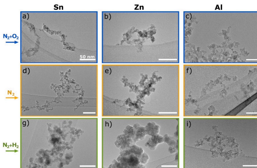
Fig. 3. TEM images of agglomerates generated from Sn, Zn, and Al electrodes in N_2 + O_2 (a-c: blue), N_2 (d-f: orange), and N_2 + H_2 (g-i: green). All scale bars are 50 nm. (For interpretation of the references to colour in this figure legend, the reader is referred to the web version of this article.)
