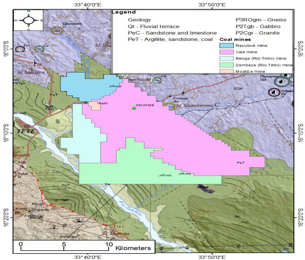
Figure 3. The Geology of Moatize in the Tete province of Mozambique.
