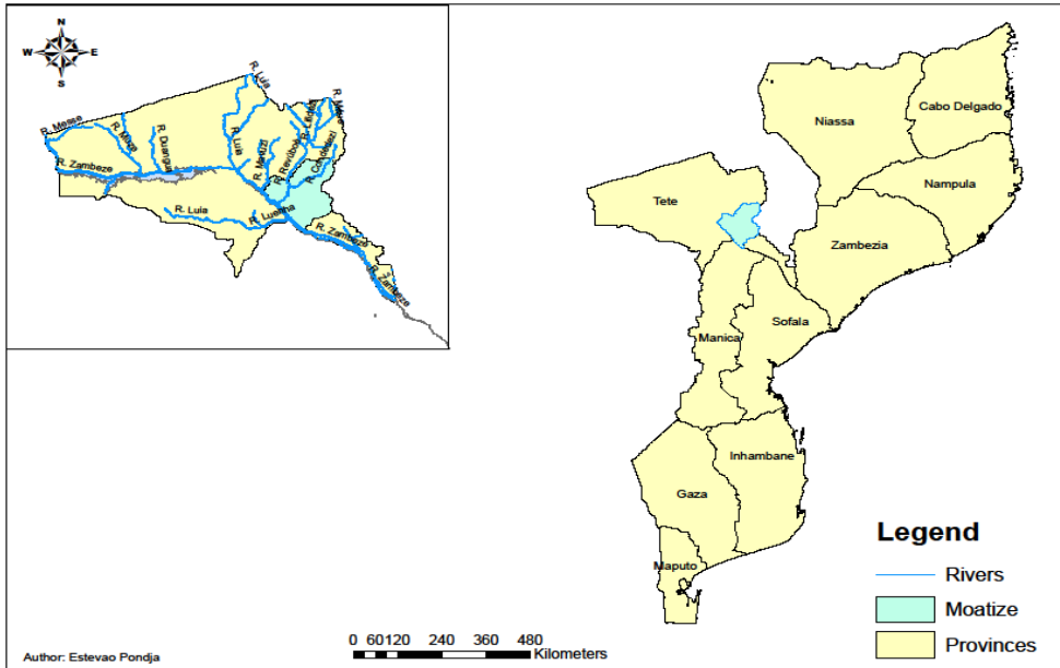
Figure 2. A map of Mozambique and of the Tete province upper left showing Moatize and various tributaries of the Zambezi River.
