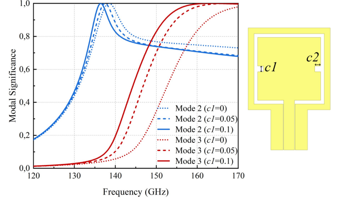
Fig. 10. Modal significance of the loop (Mode 2) and patch (Mode 3) with different slot lengths. Loop-patch structure with two slots etched on the patch shown to the right.
