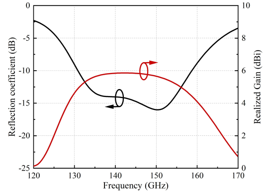
Fig. 9. Reflection coefficient and realized gain of loop-patch antenna.
