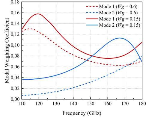
Fig. 5. Modal weighting coefficient in Fig. 3 of two modes of interest for two different W_g 's.
